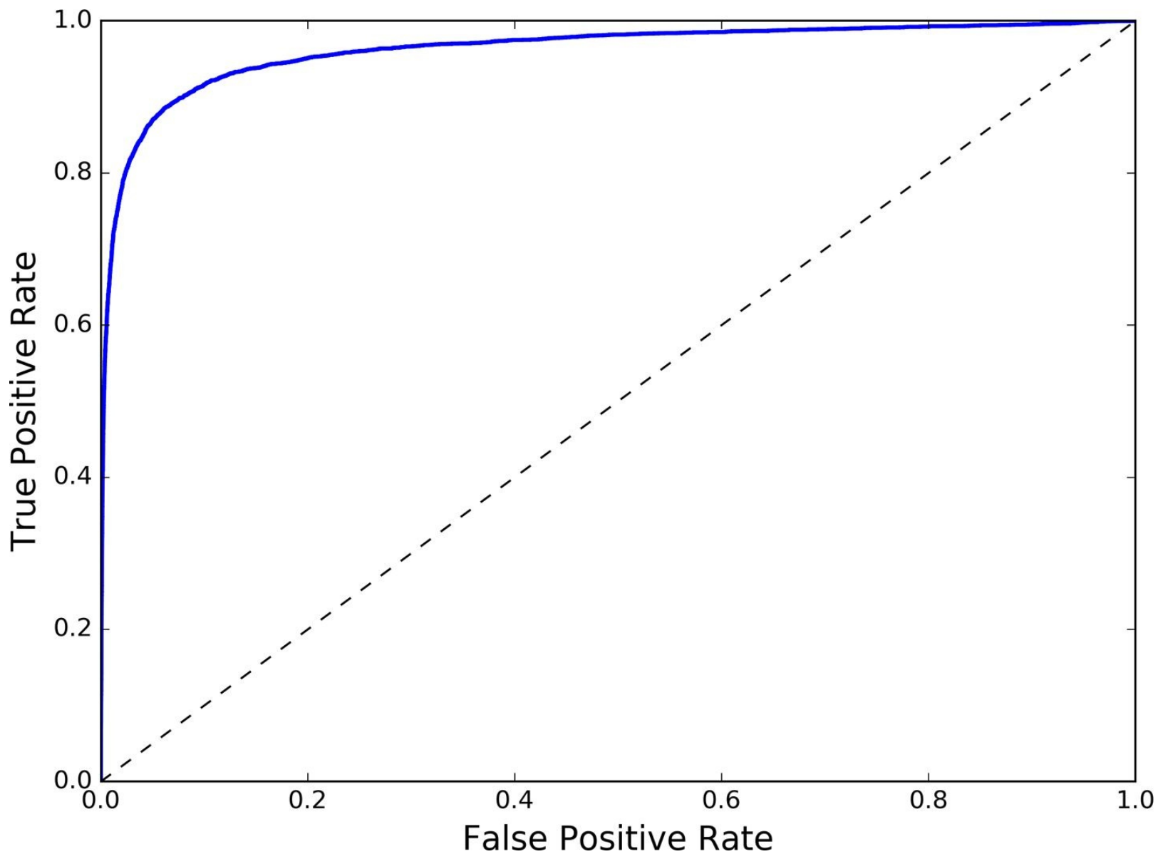
Figure 3-6. ROC curve
