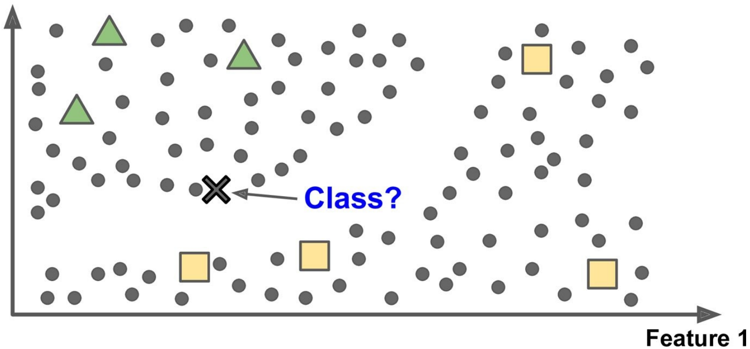
Figure 1-11. Semisupervised learning
