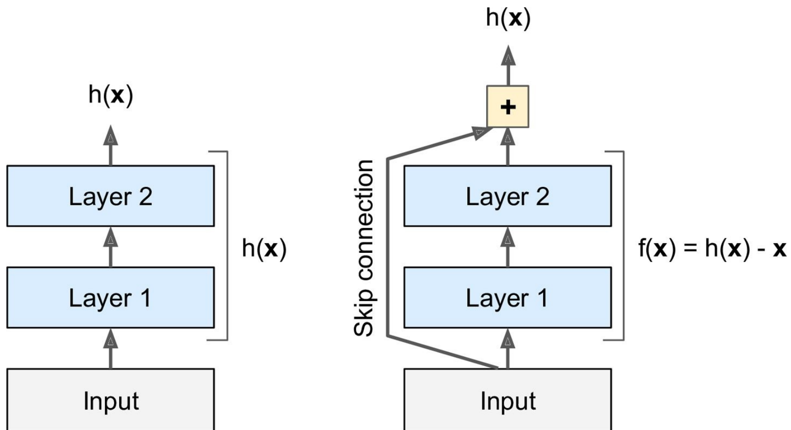
Figure 13-12. Residual learning
