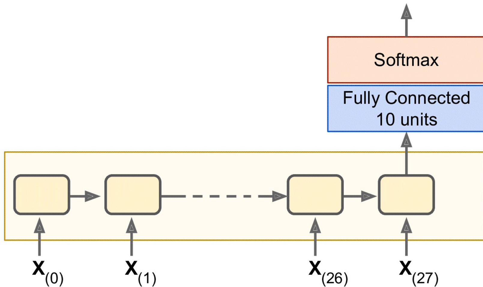
Figure 14-6. Sequence classifier
