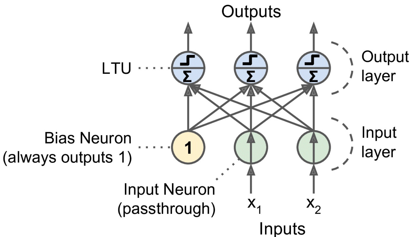
Figure 10-5. Perceptron diagram
