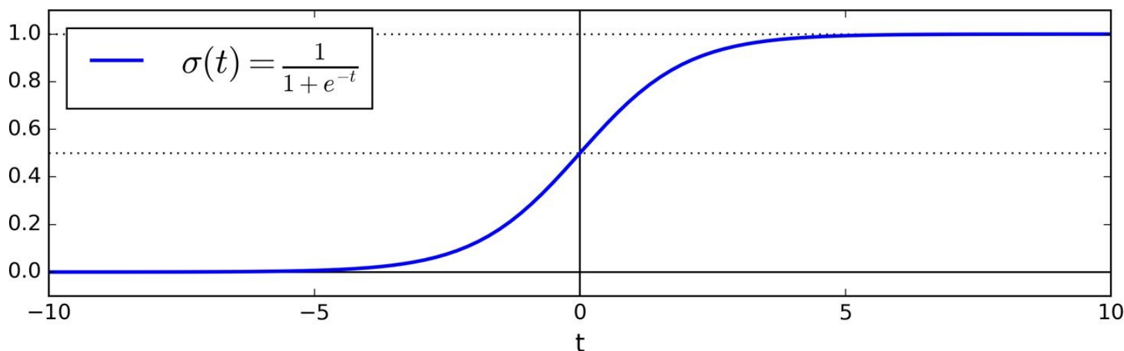
Figure 4-21. Logistic function
