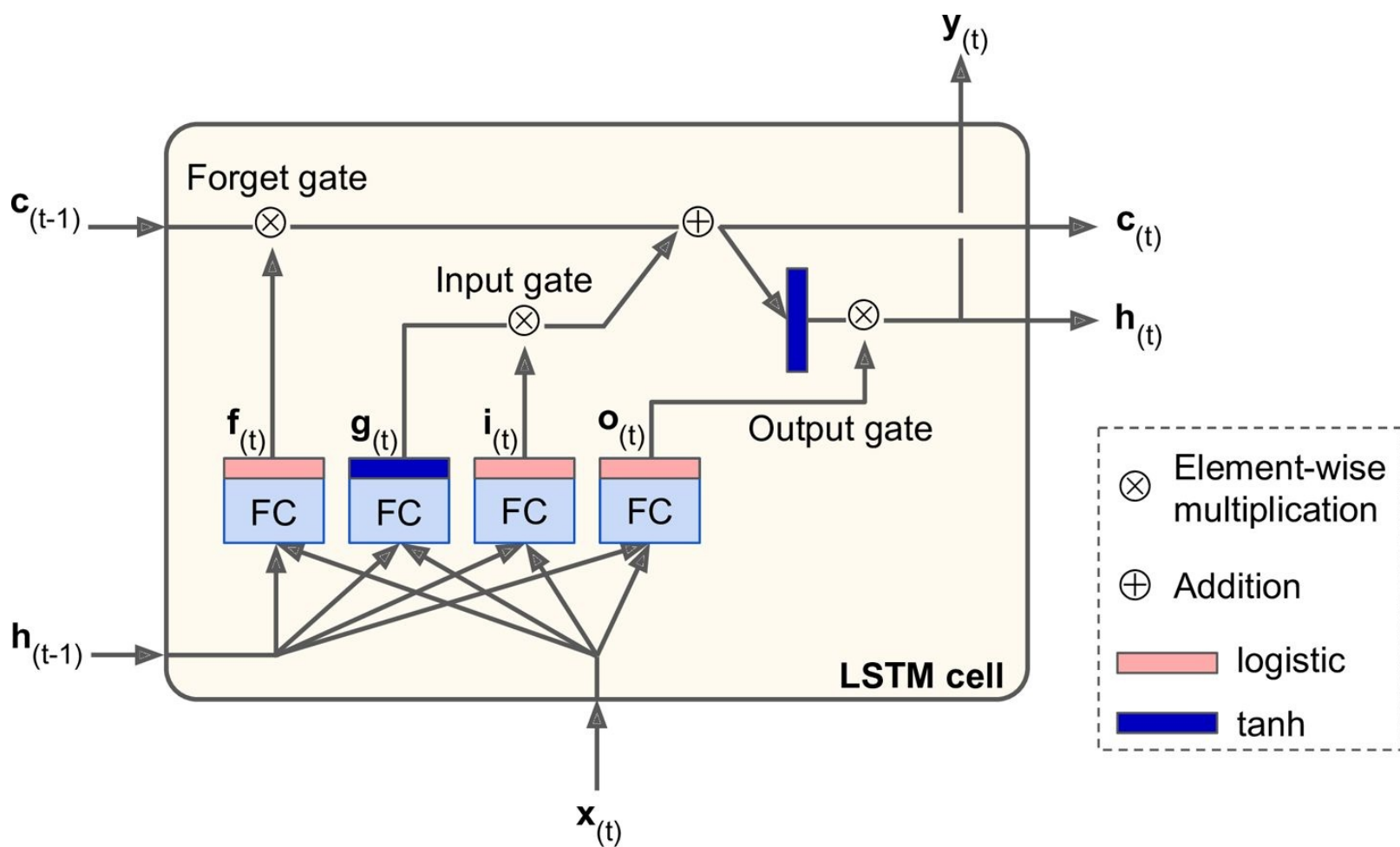
Figure 14-13. LSTM cell
