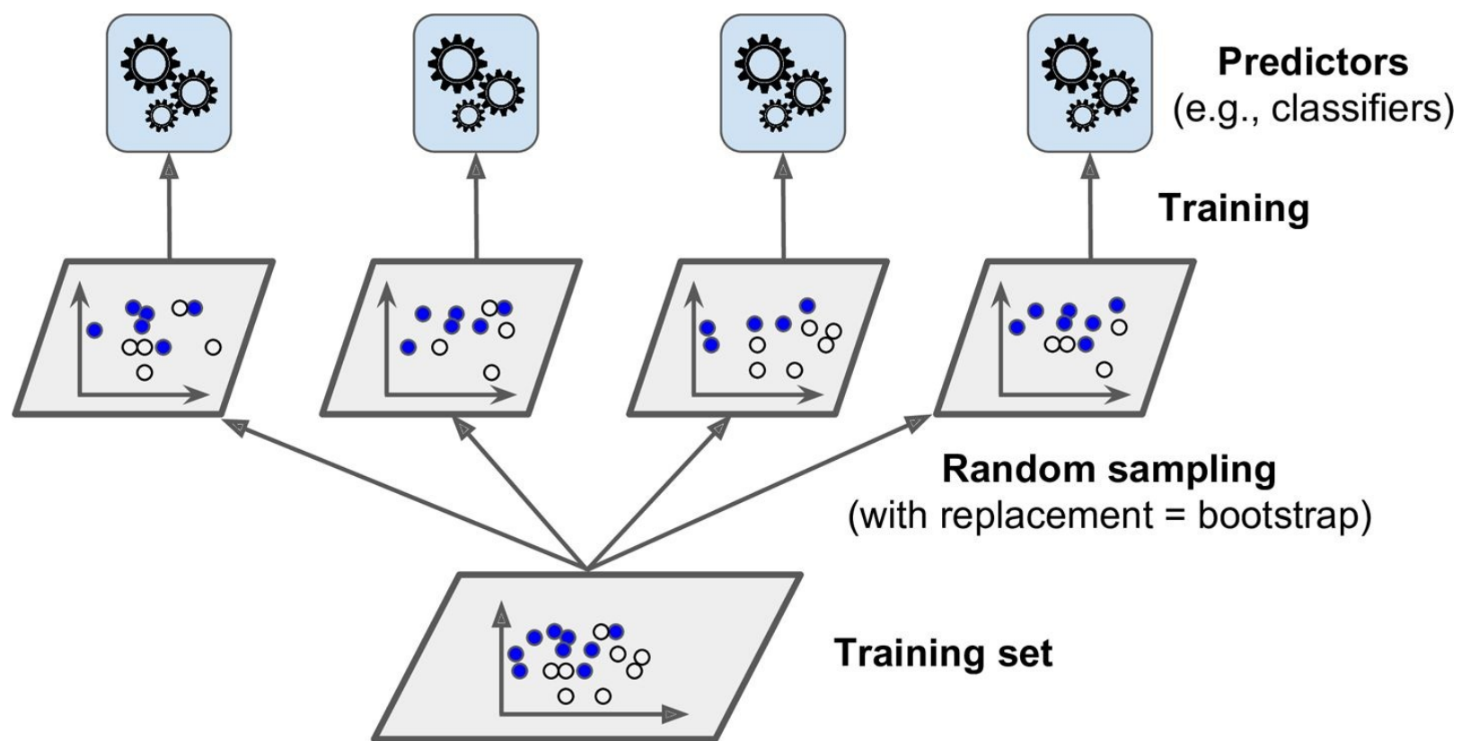
Figure 7-4. Pasting/bagging training set sampling and training
