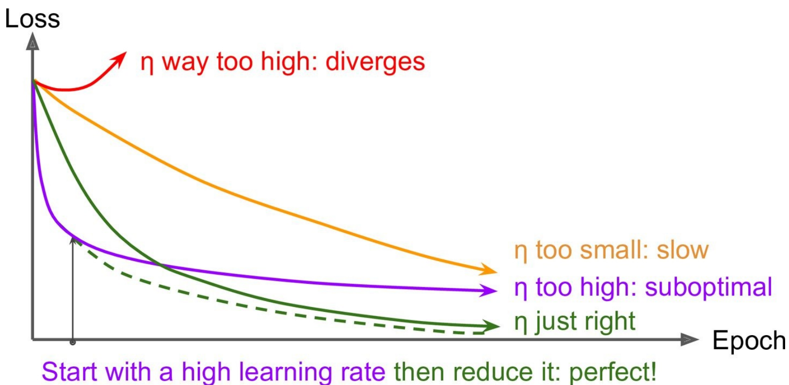
Figure 11-8. Learning curves for various learning rates \eta
