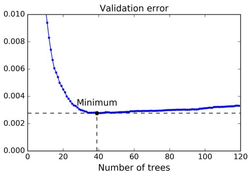
Figure 7-11. Tuning the number of trees using early stopping
