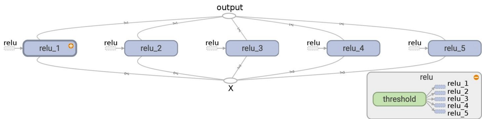
Figure 9-8. Five ReLUs sharing the threshold variable
