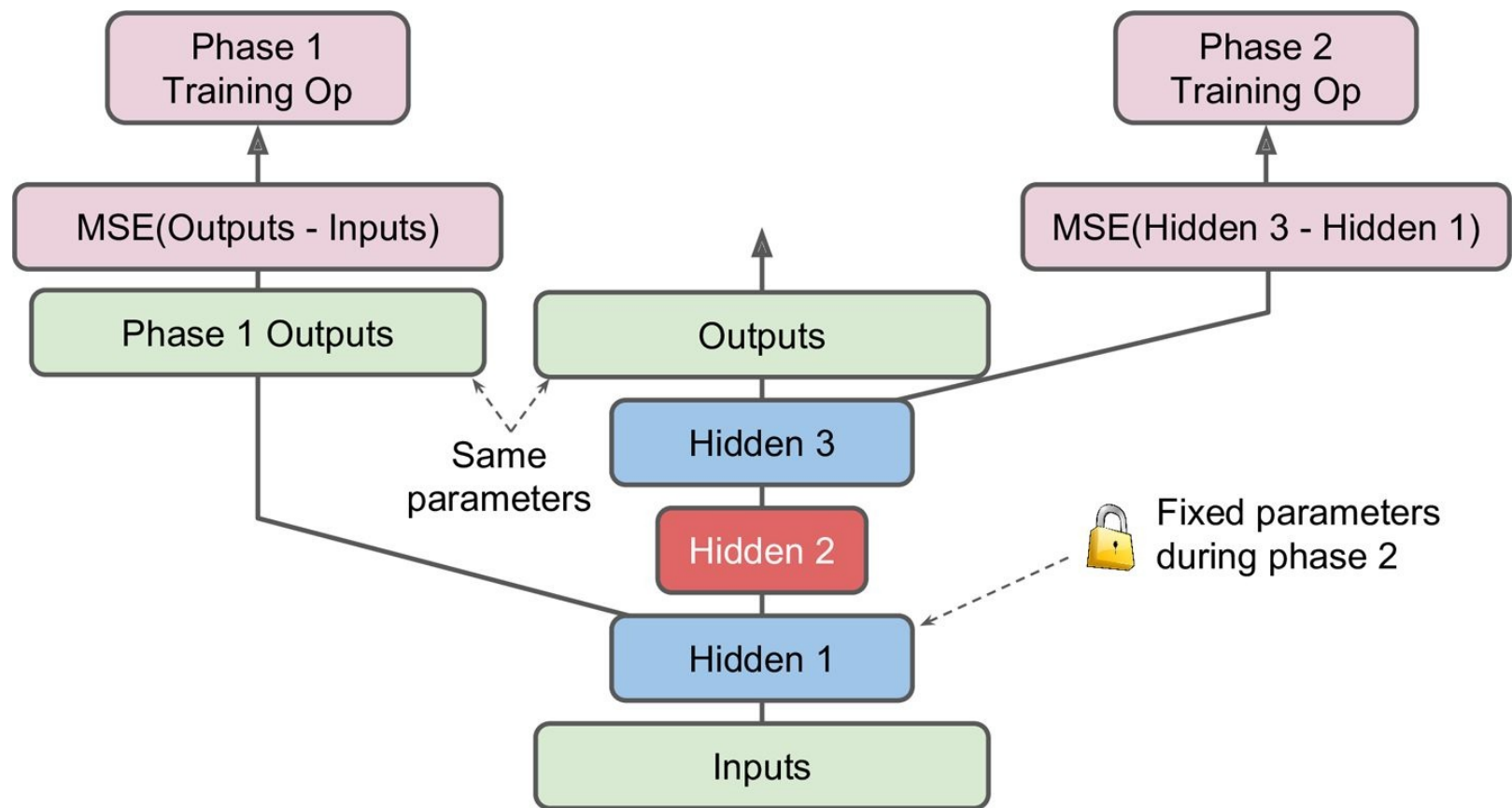
Figure 15-5. A single graph to train a stacked autoencoder
