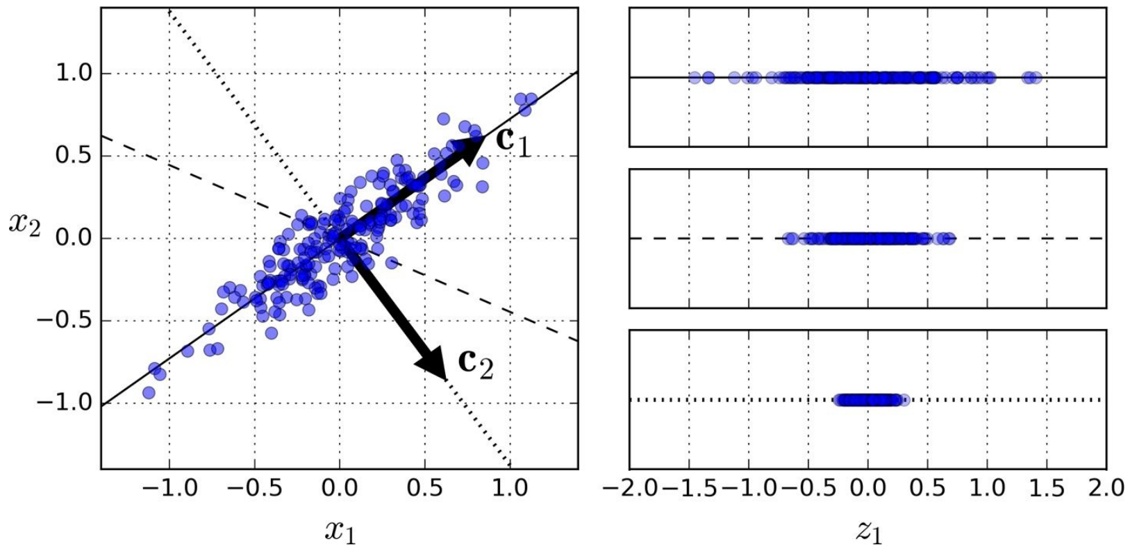
Figure 8-7. Selecting the subspace onto which to project
