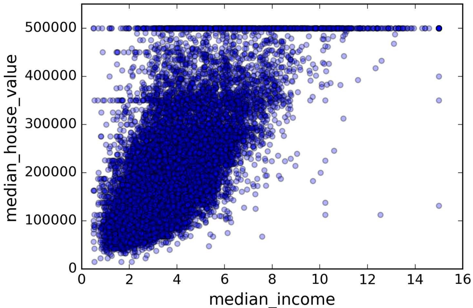
Figure 2-16. Median income versus median house value
