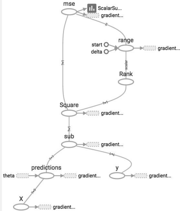
Figure 9-4. Visualizing the graph using TensorBoard
