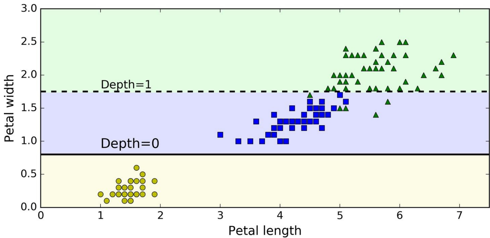
Figure 6-8. Sensitivity to training set details
