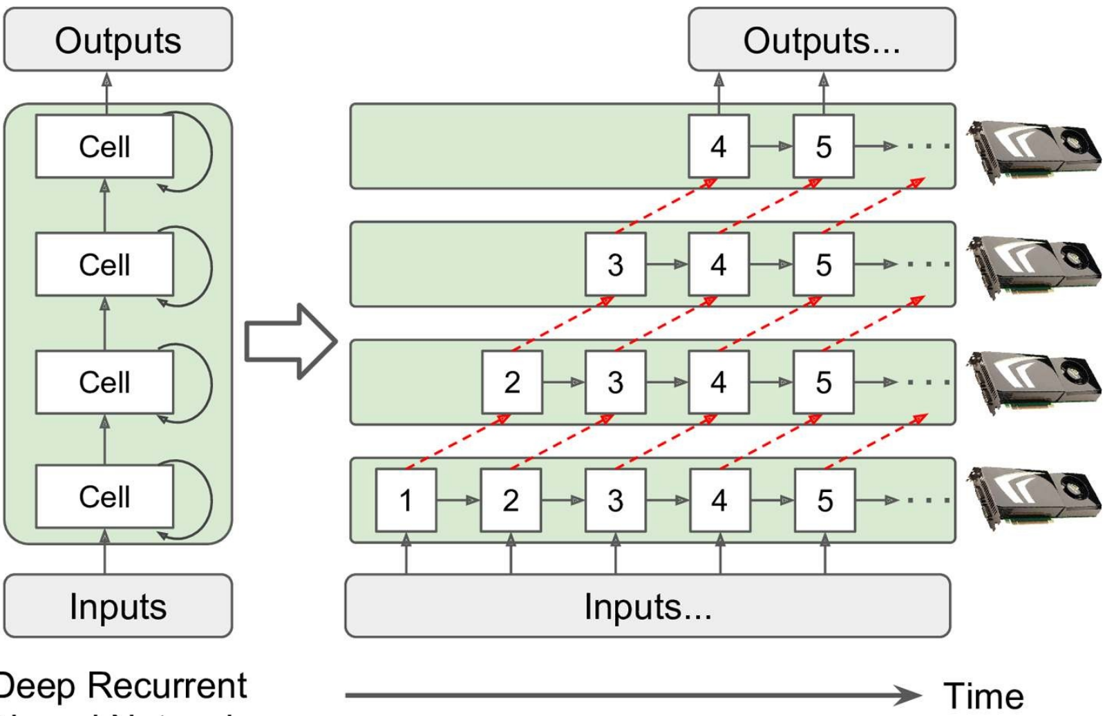
Figure 12-16. Splitting a deep recurrent neural network
