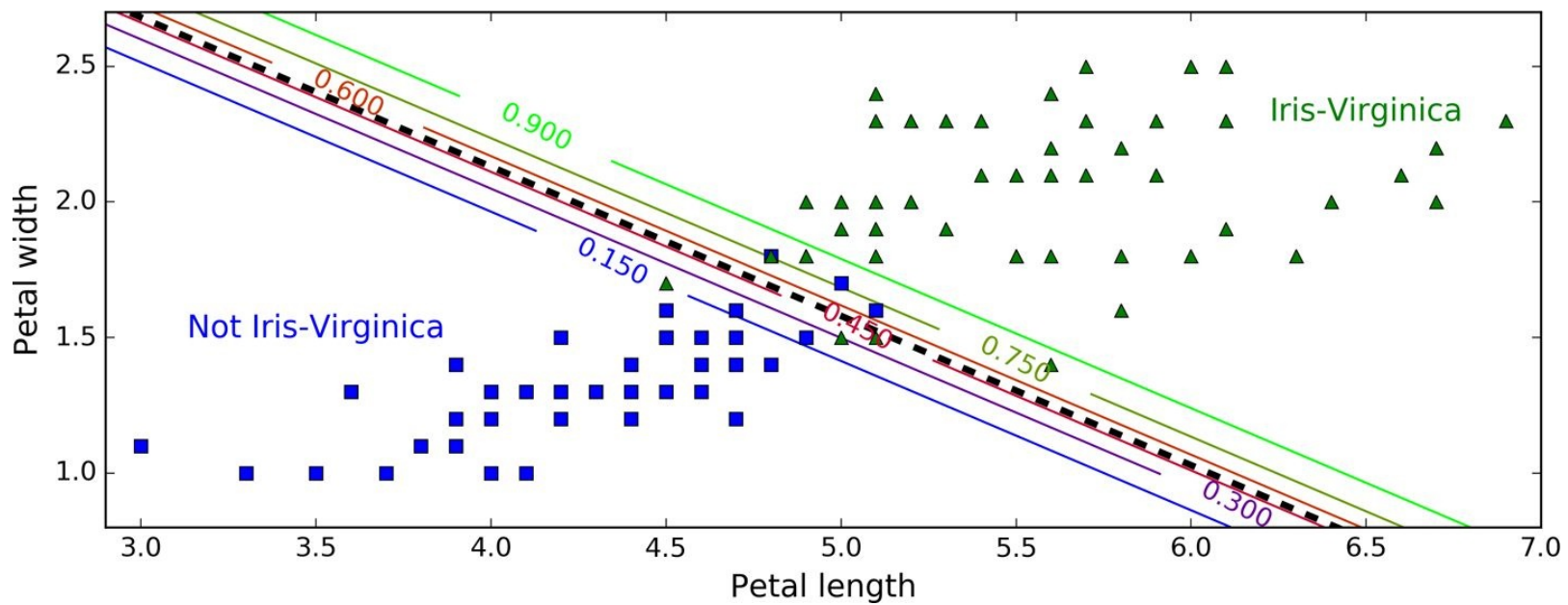
Figure 4-24. Linear decision boundary
