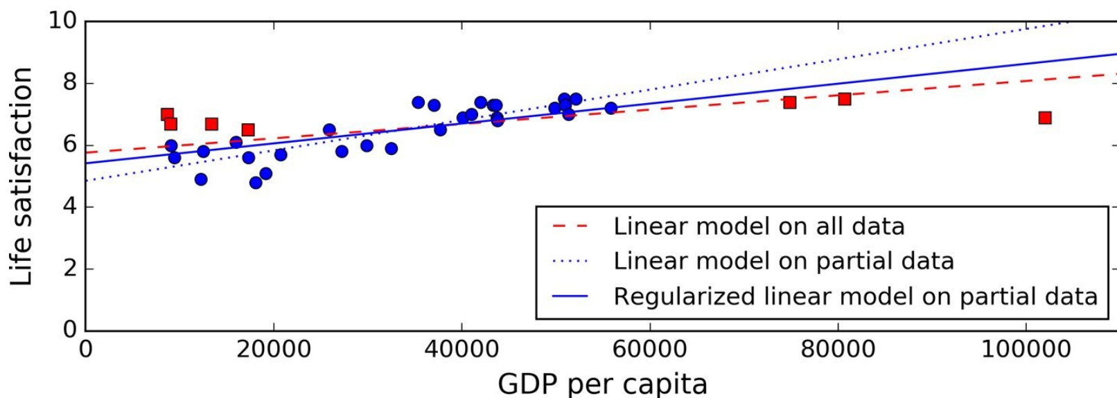
Figure 1-23. Regularization reduces the risk of overfitting
