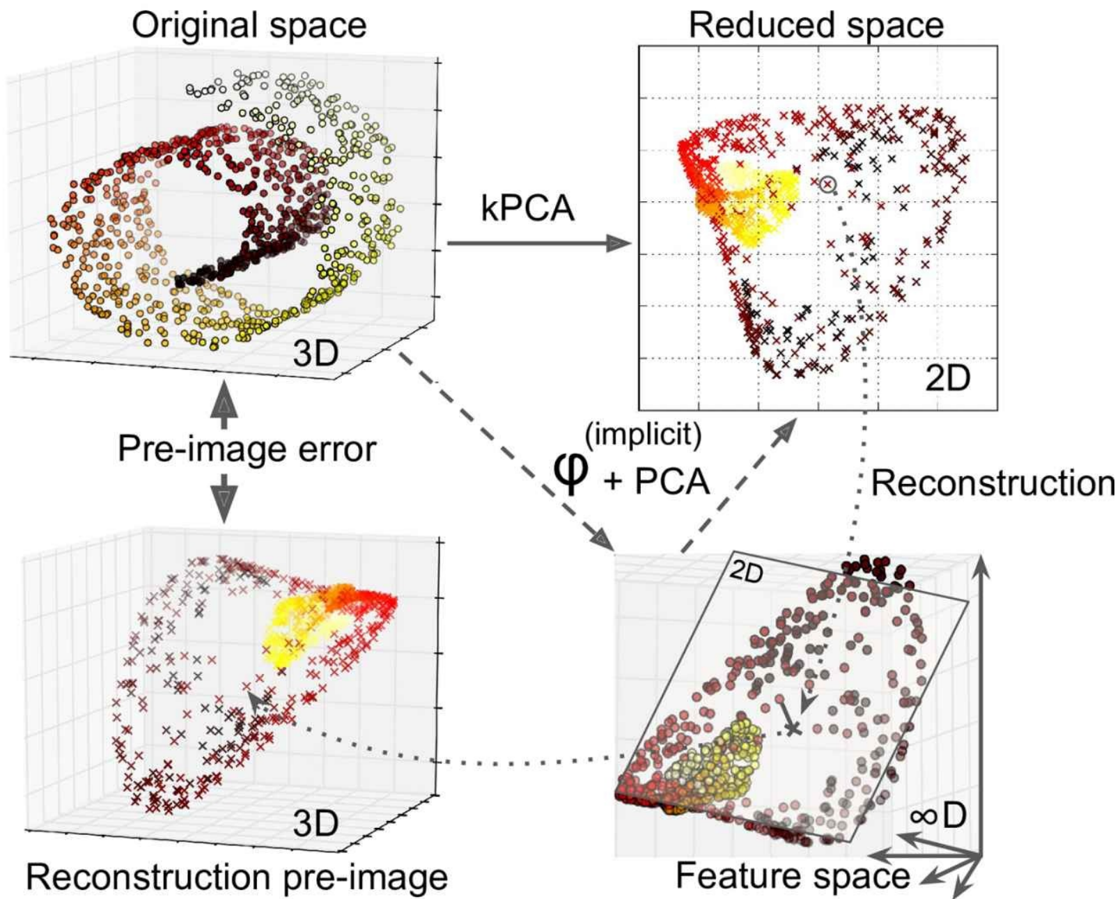
Figure 8-11. Kernel PCA and the reconstruction pre-image error
