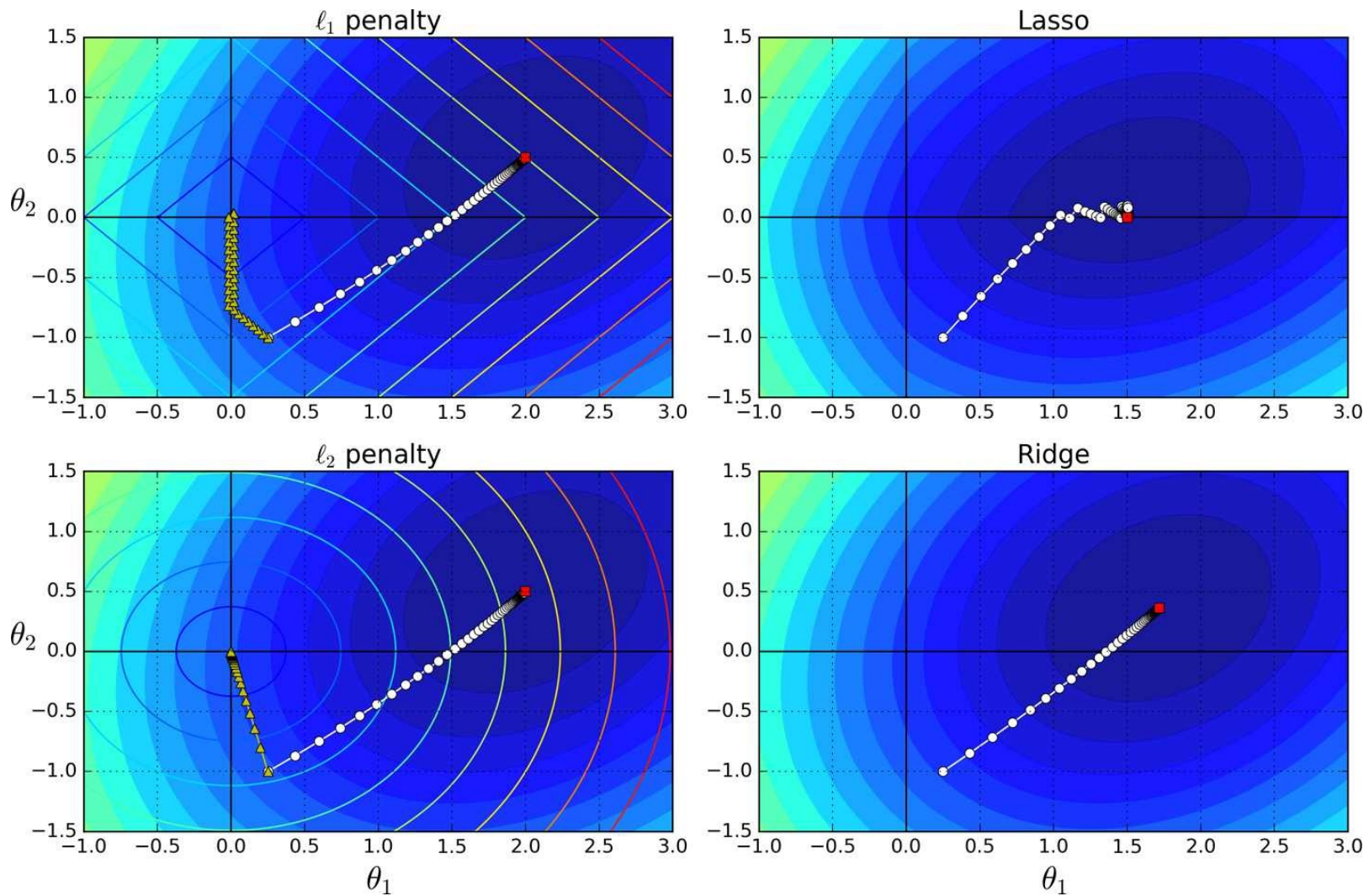
Figure 4-19. Lasso versus Ridge regularization
