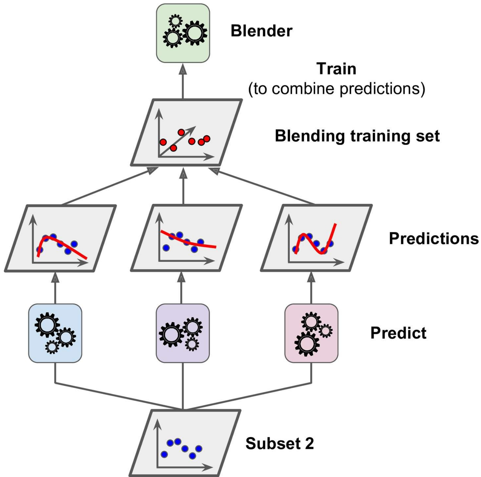
Figure 7-14. Training the blender
