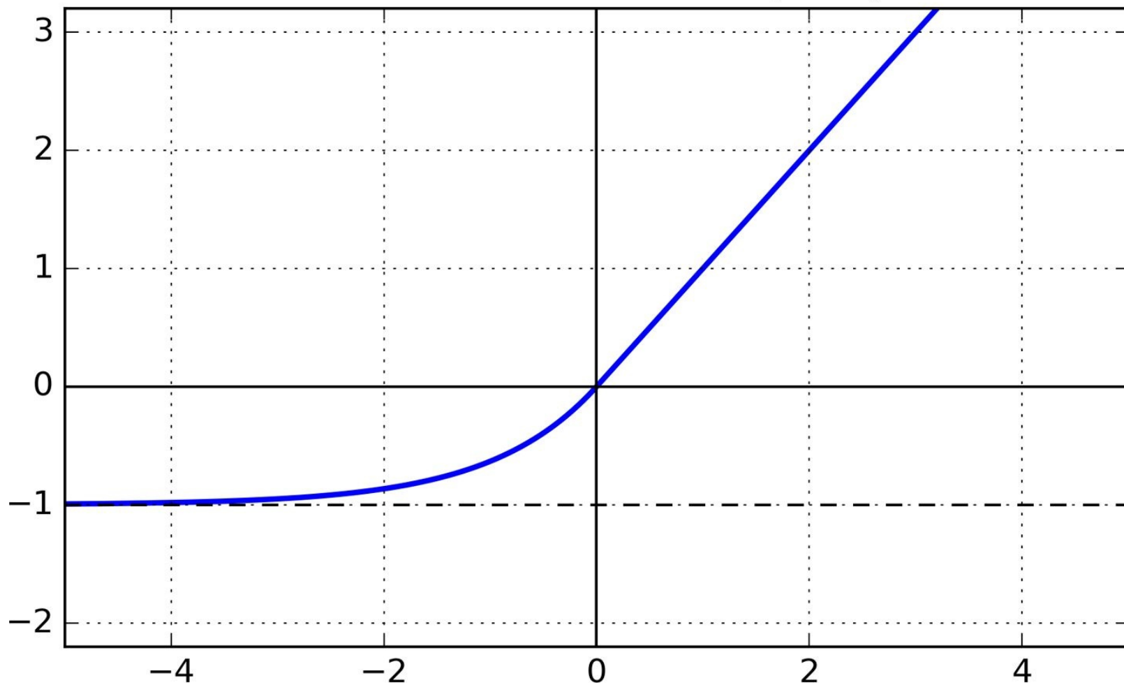
Figure 11-3. ELU activation function
