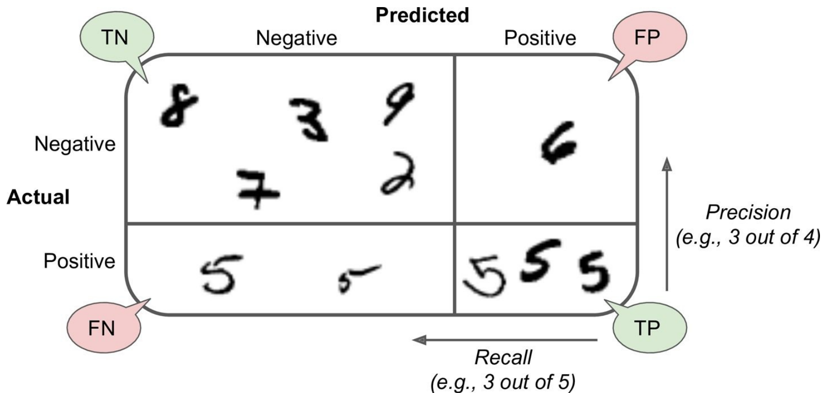
Figure 3-2. An illustrated confusion matrix
