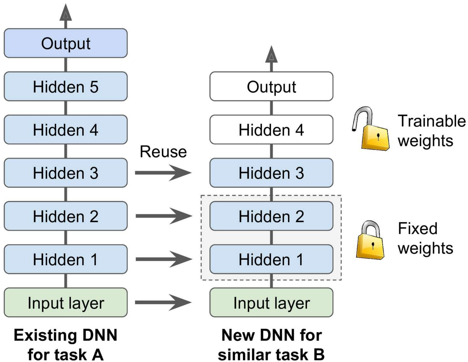
Figure 11-4. Reusing pretrained layers
