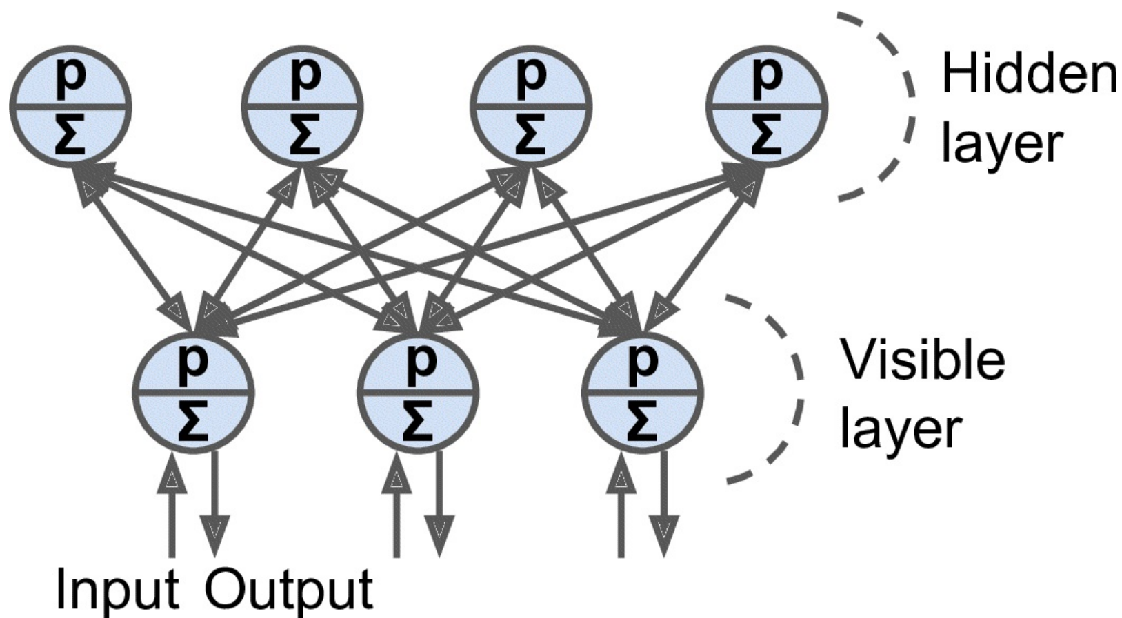
Figure E-3. Restricted Boltzmann machine
