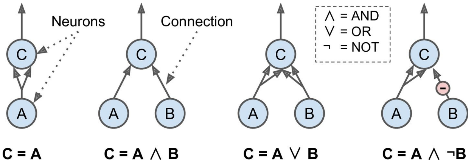
Figure 10-3. ANNs performing simple logical computations
