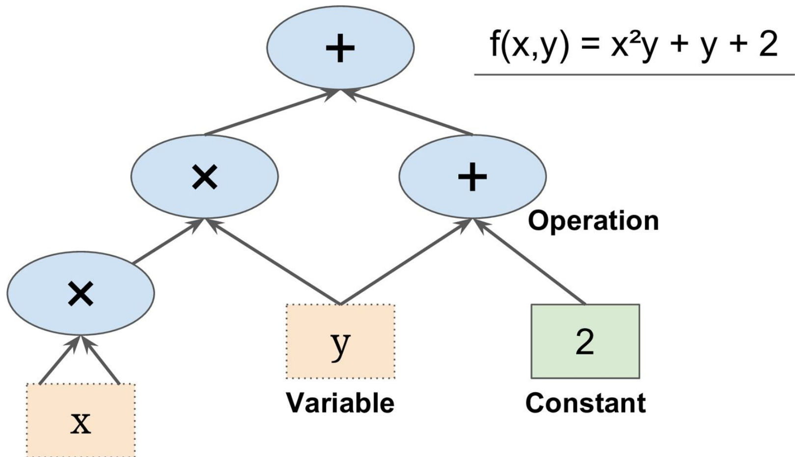
Figure 9-1. A simple computation graph
