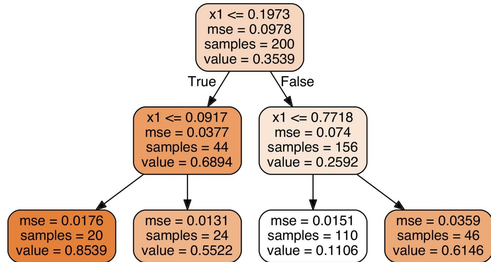
Figure 6-4. A Decision Tree for regression
