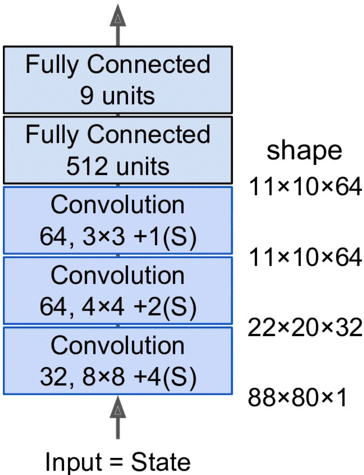
Figure 16-10. Deep Q-network to play Ms. Pac-Man
