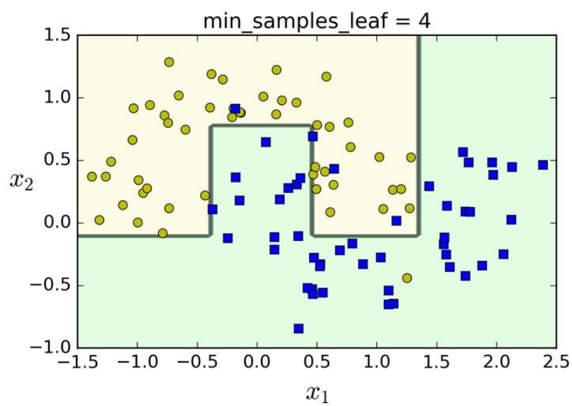
Figure 6-3. Regularization using min_samples_leaf
