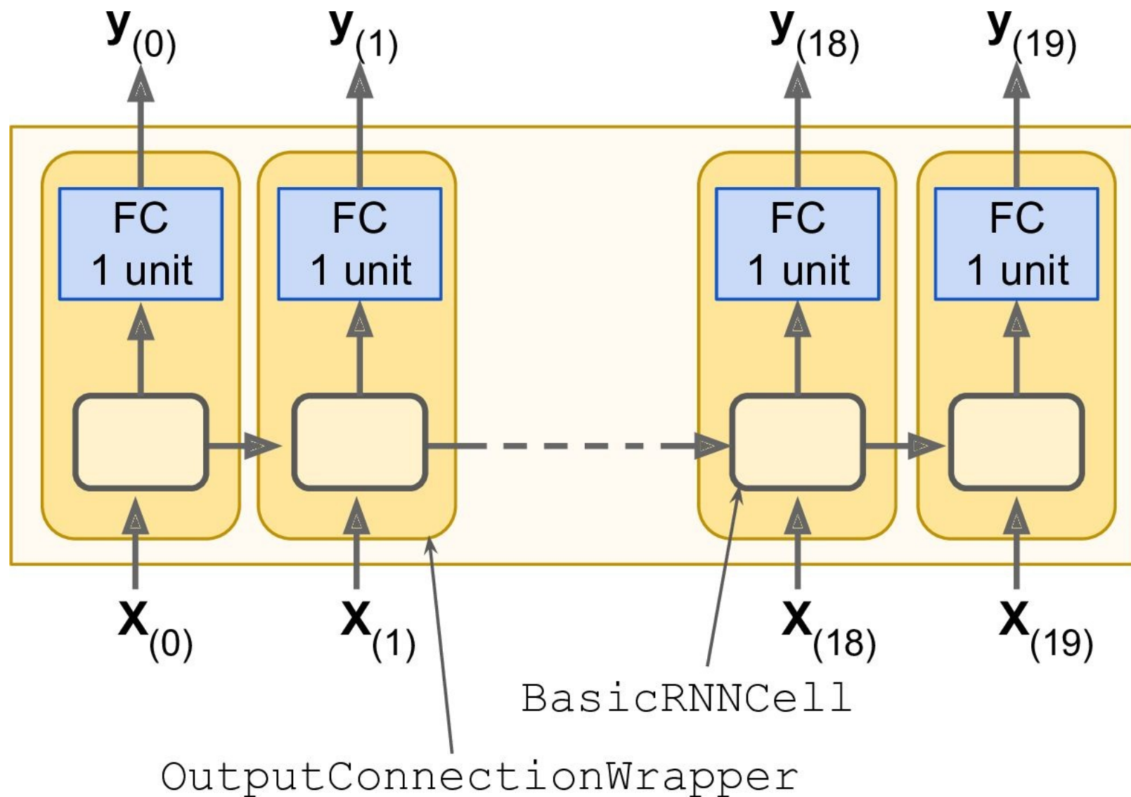
Figure 14-8. RNN cells using output projections
