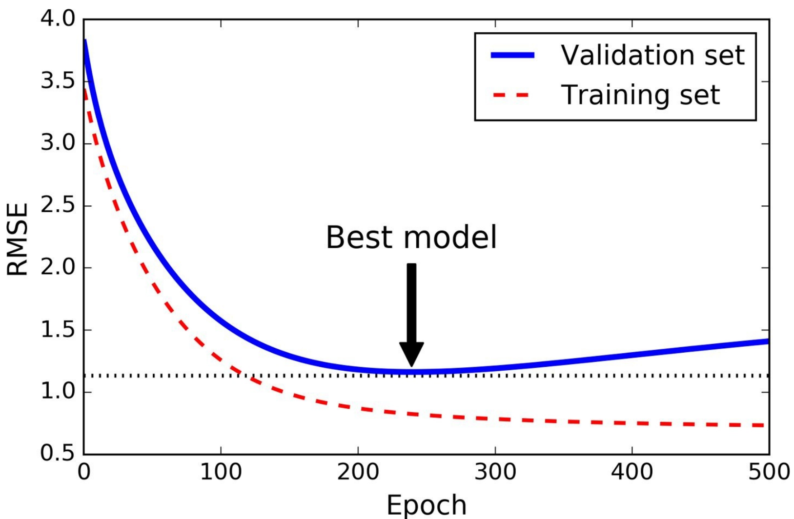
Figure 4-20. Early stopping regularization
