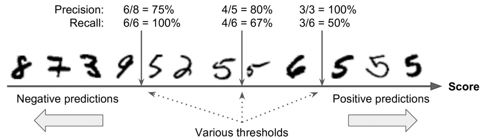
Figure 3-3. Decision threshold and precision/recall tradeoff
