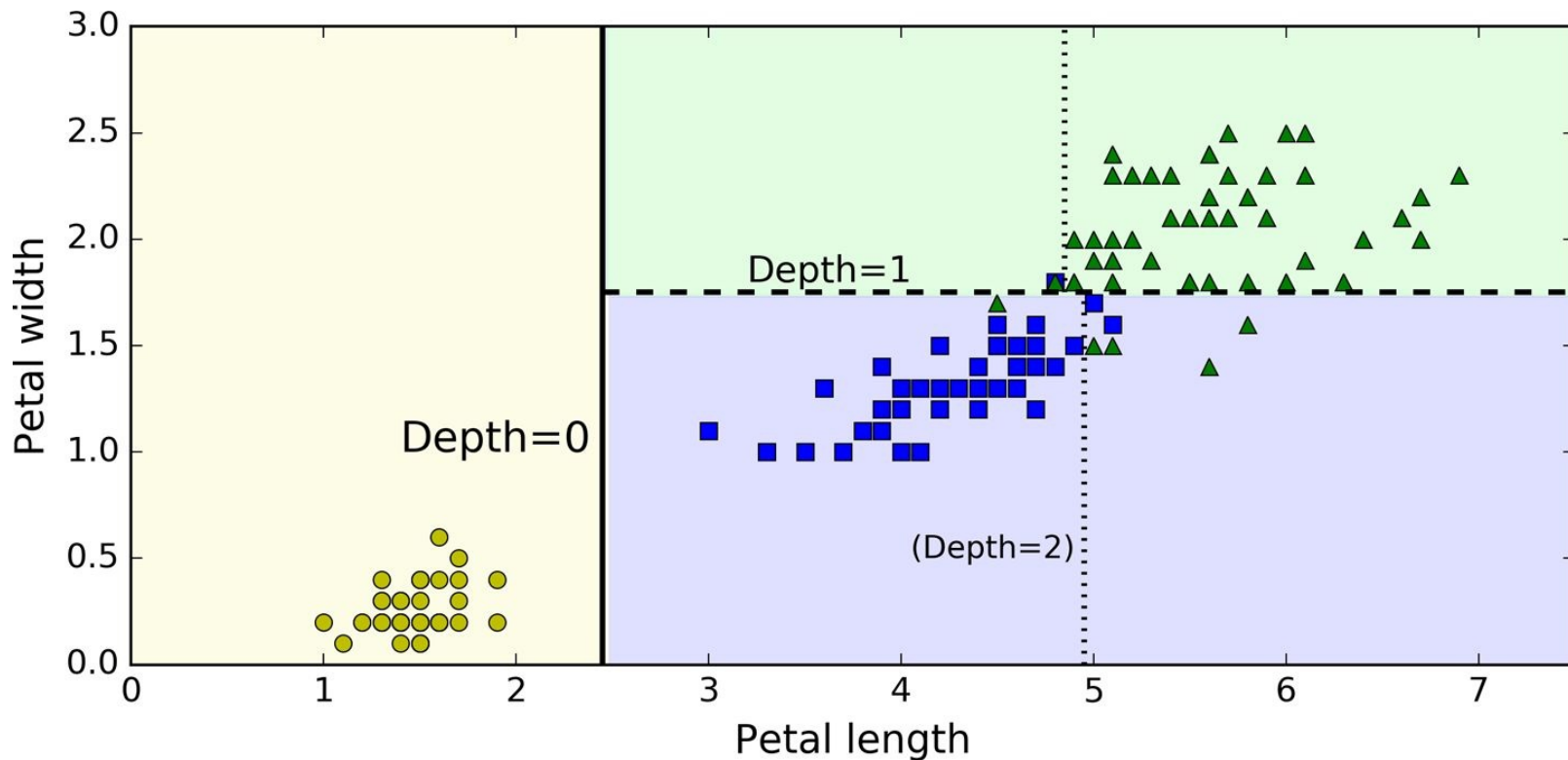
Figure 6-2. Decision Tree decision boundaries
