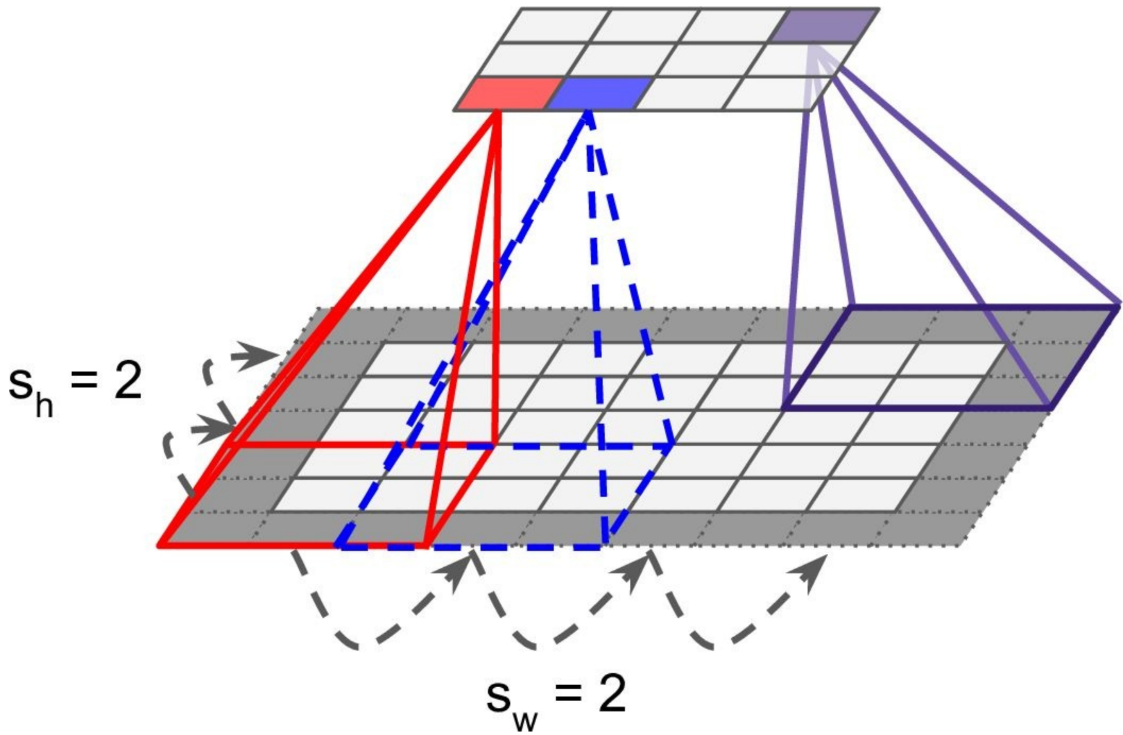
Figure 13-4. Reducing dimensionality using a stride
