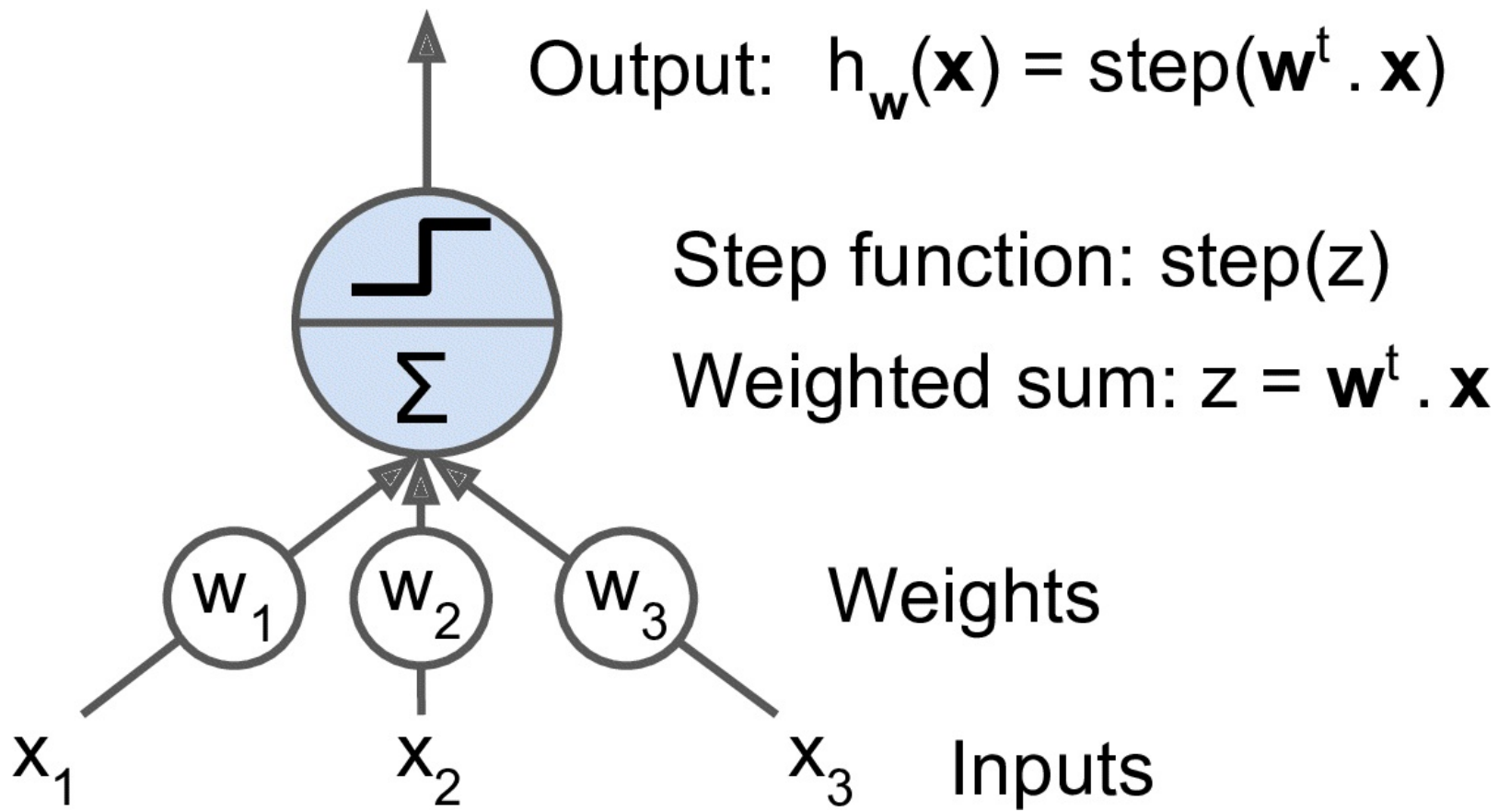
Figure 10-4. Linear threshold unit
