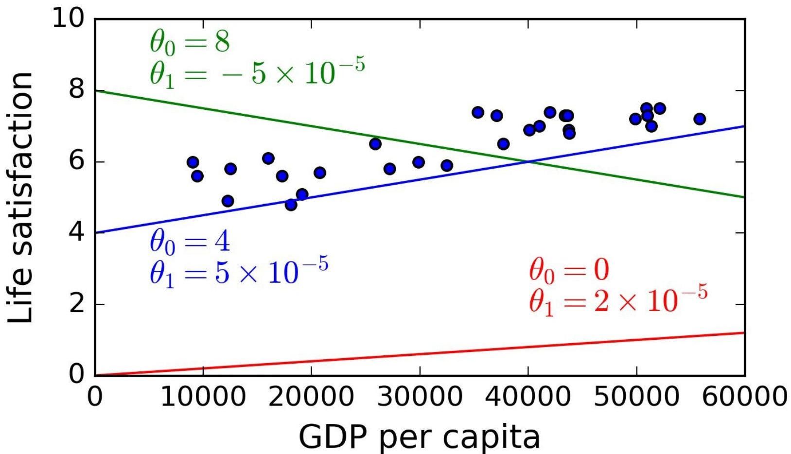
Figure 1-18. A few possible linear models
