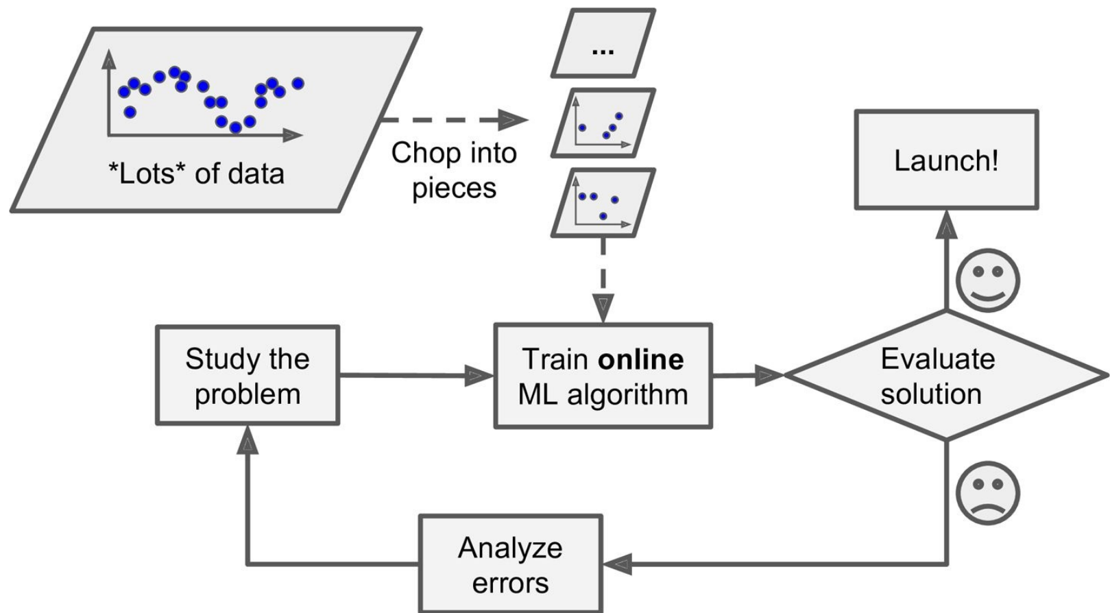
Figure 1-14. Using online learning to handle huge datasets
