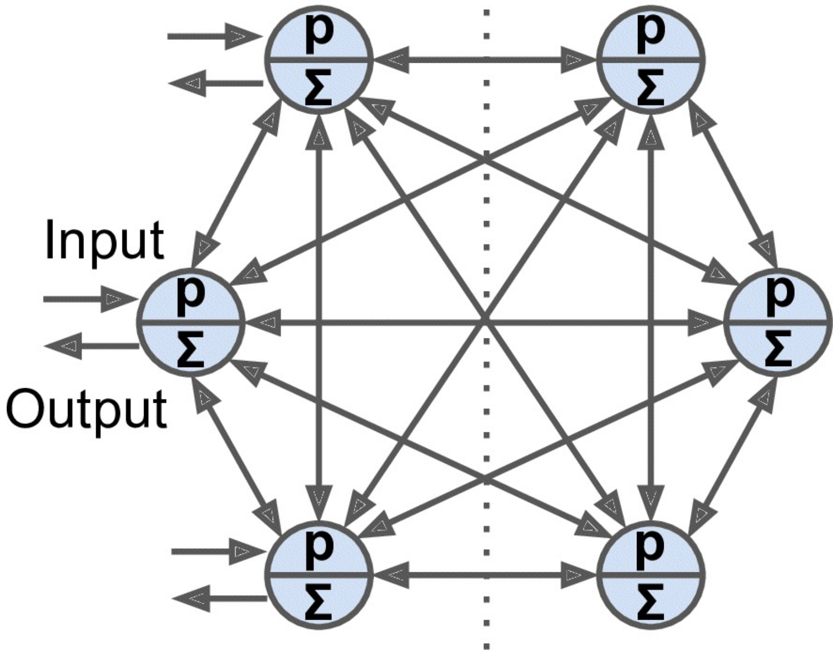
Figure E-2. Boltzmann machine
