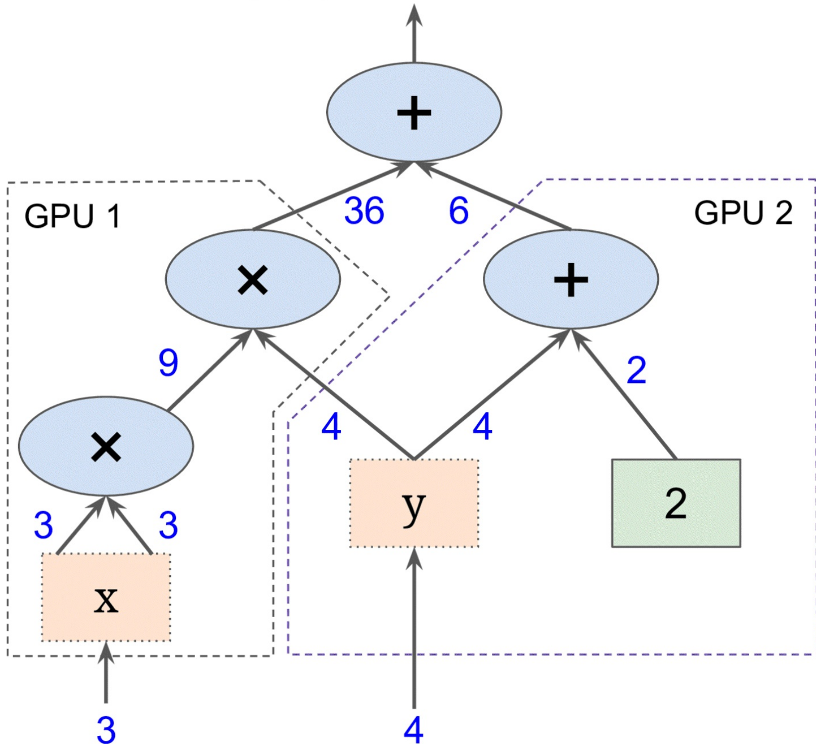
Figure 9-2. Parallel computation on multiple CPUs/GPUs/servers
