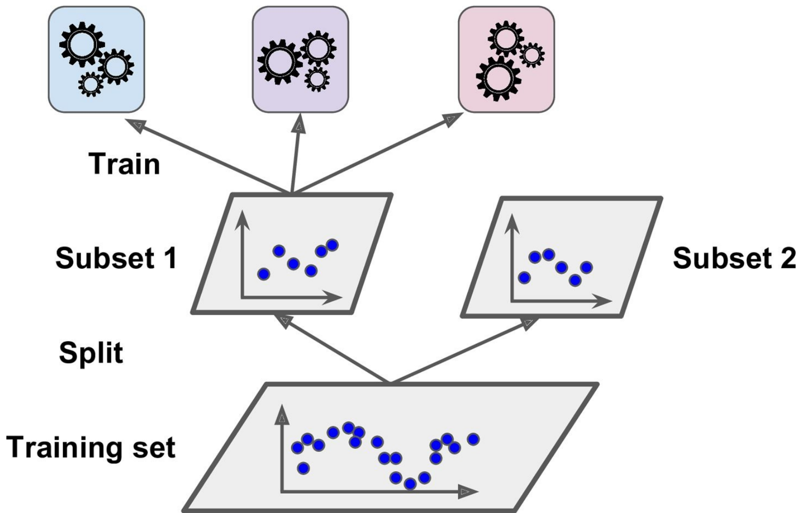
Figure 7-13. Training the first layer
