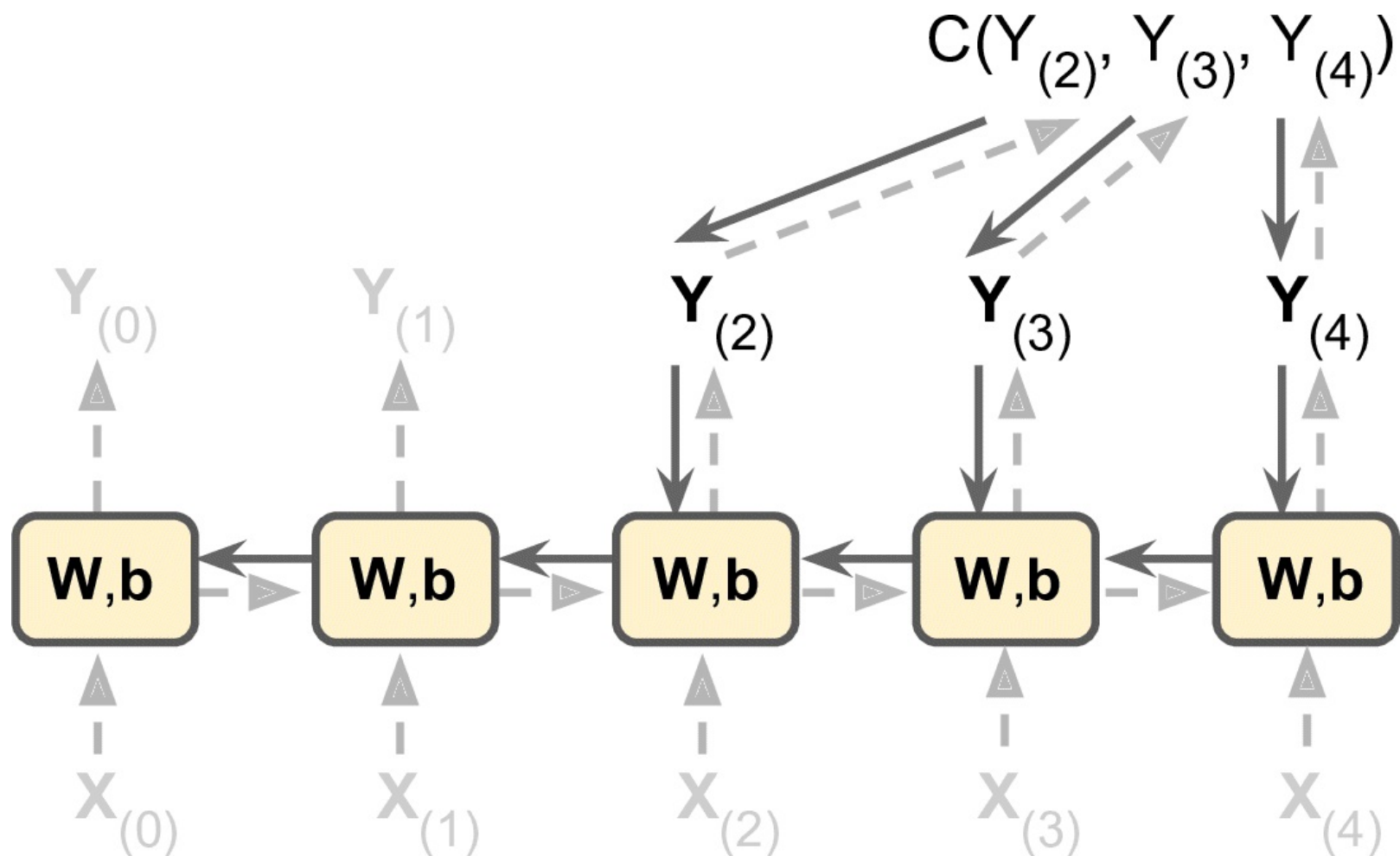
Figure 14-5. Backpropagation through time
