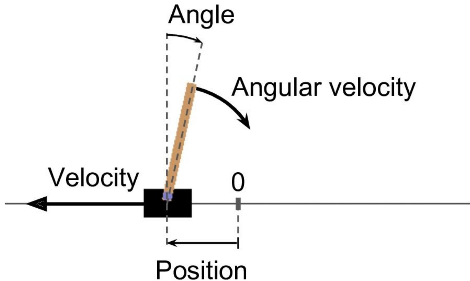
Figure 16-4. The CartPole environment
