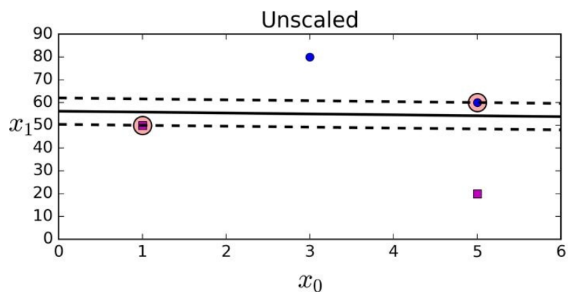
Figure 5-2. Sensitivity to feature scales
