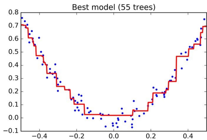
Figure 7-11. Tuning the number of trees using early stopping
