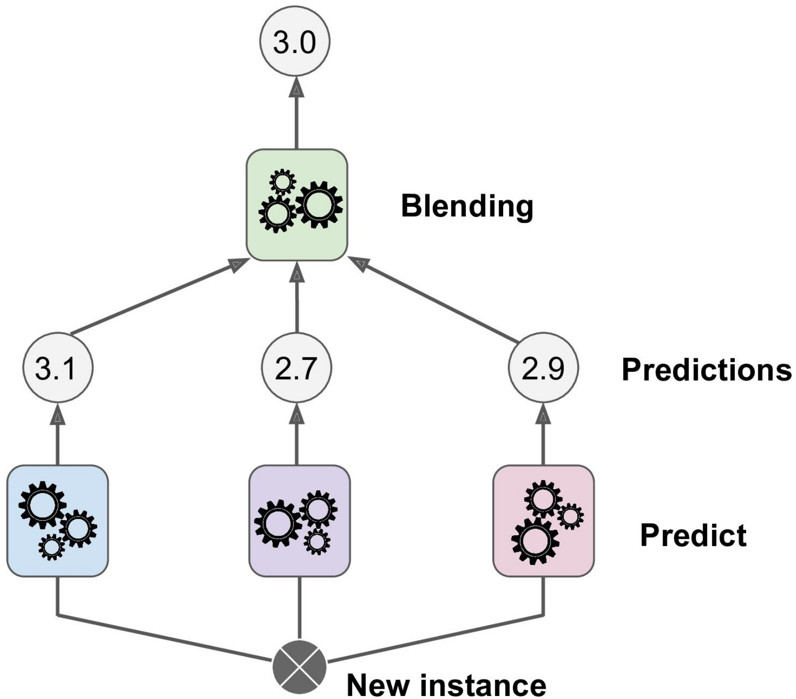
Figure 7-12. Aggregating predictions using a blending predictor
