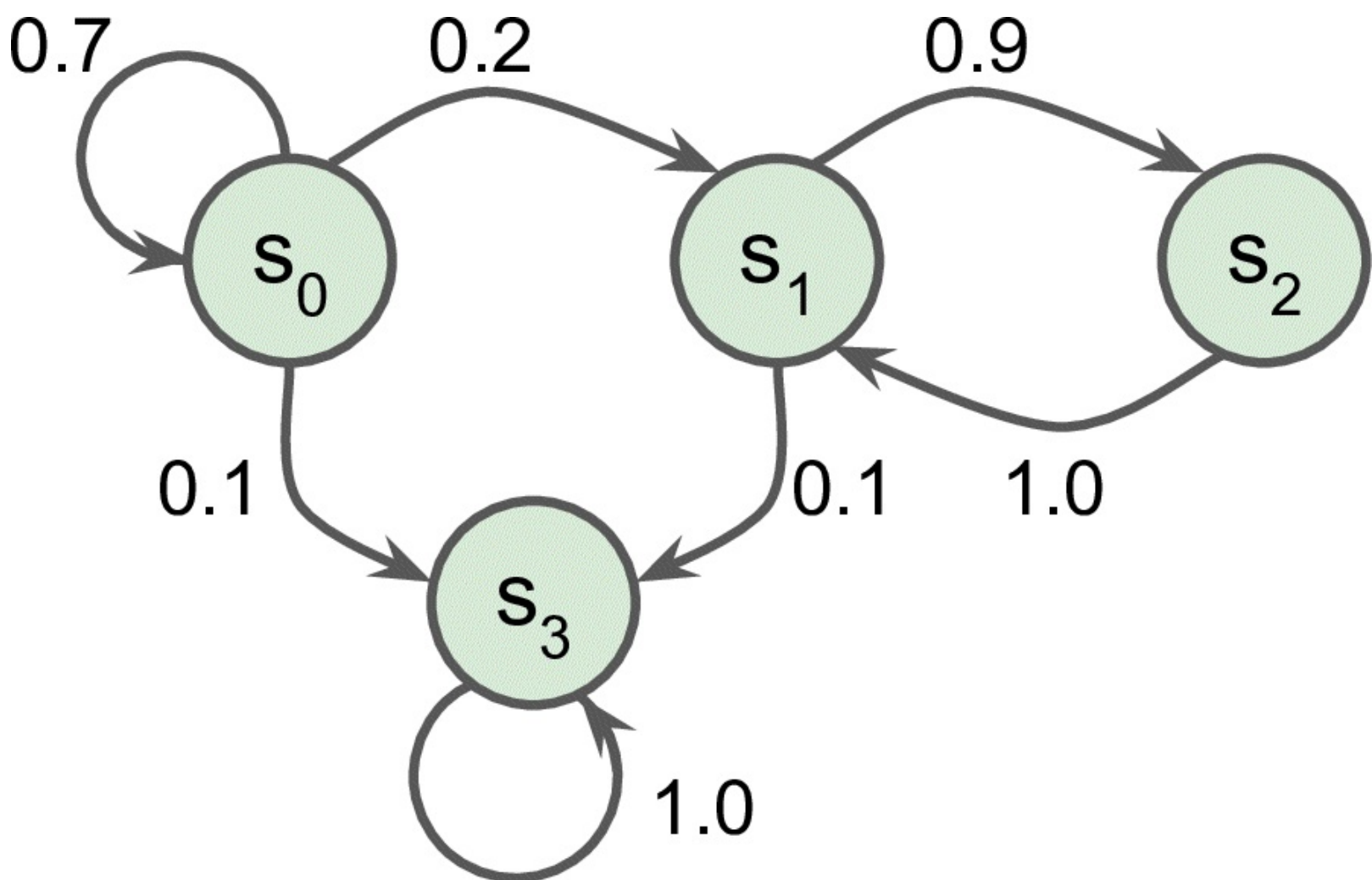
Figure 16-7. Example of a Markov chain
