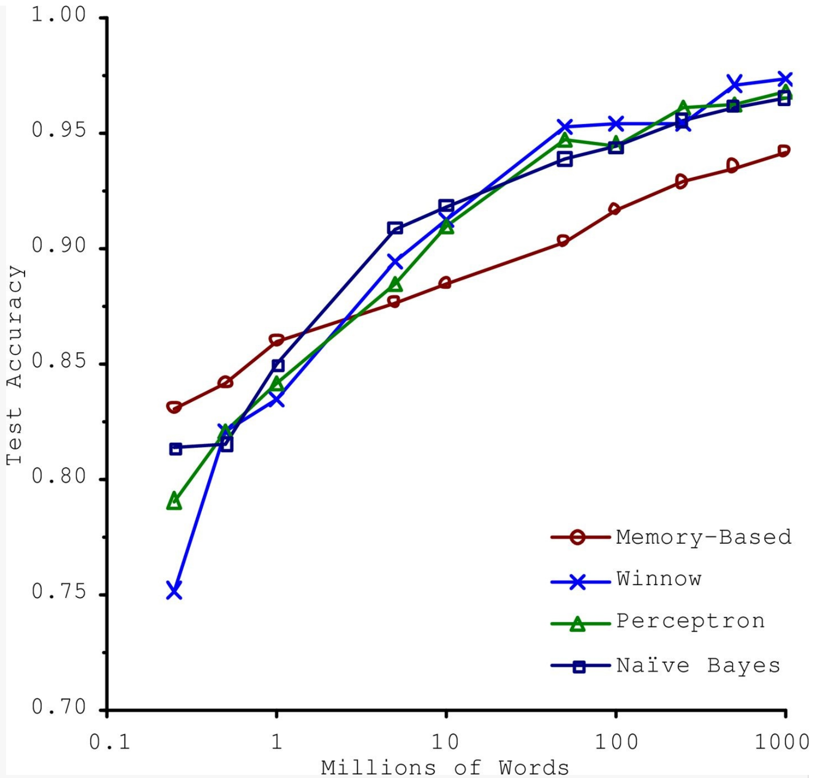
Figure 1-20. The importance of data versus algorithms 9
