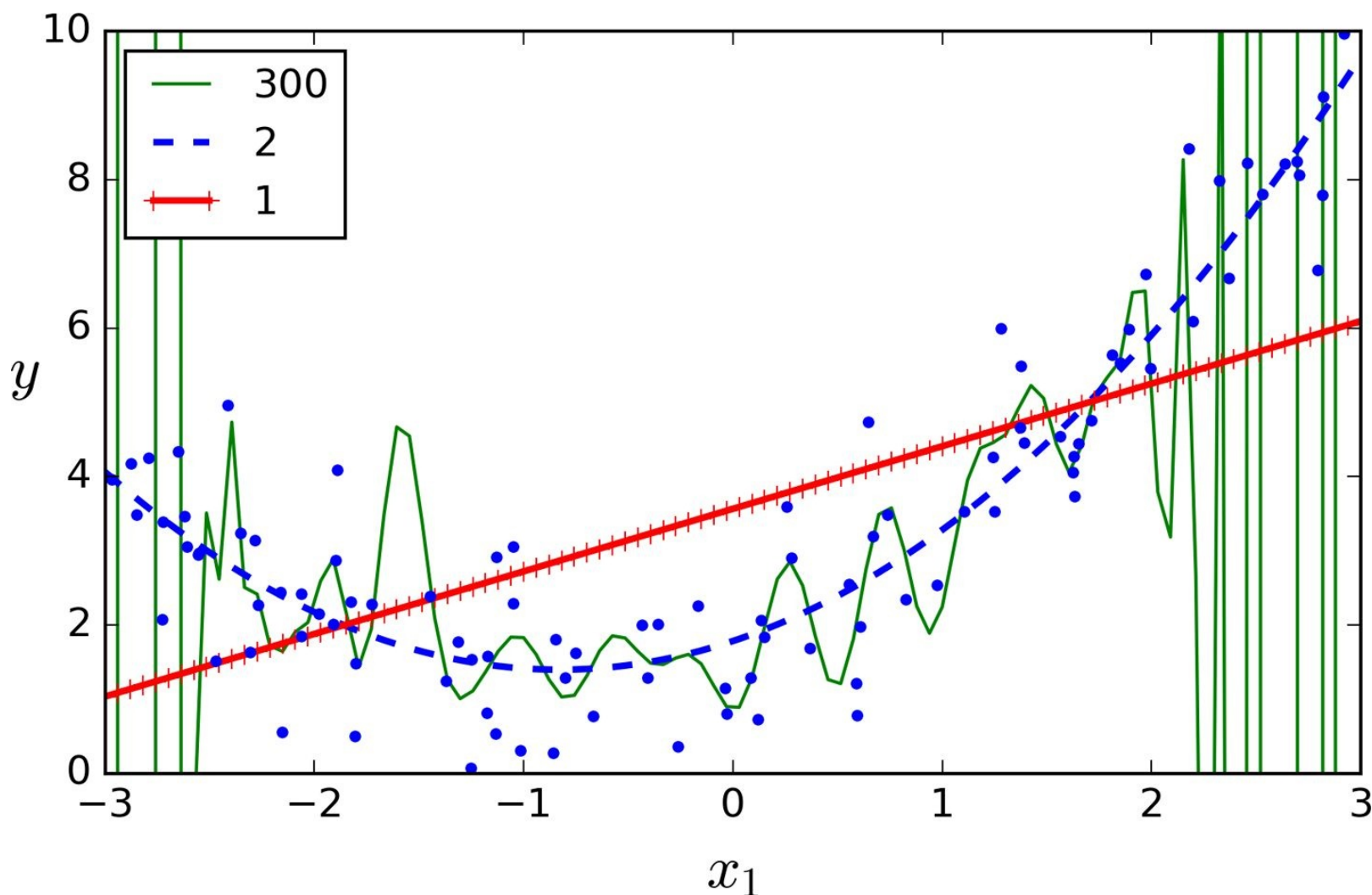
Figure 4-14. High-degree Polynomial Regression
