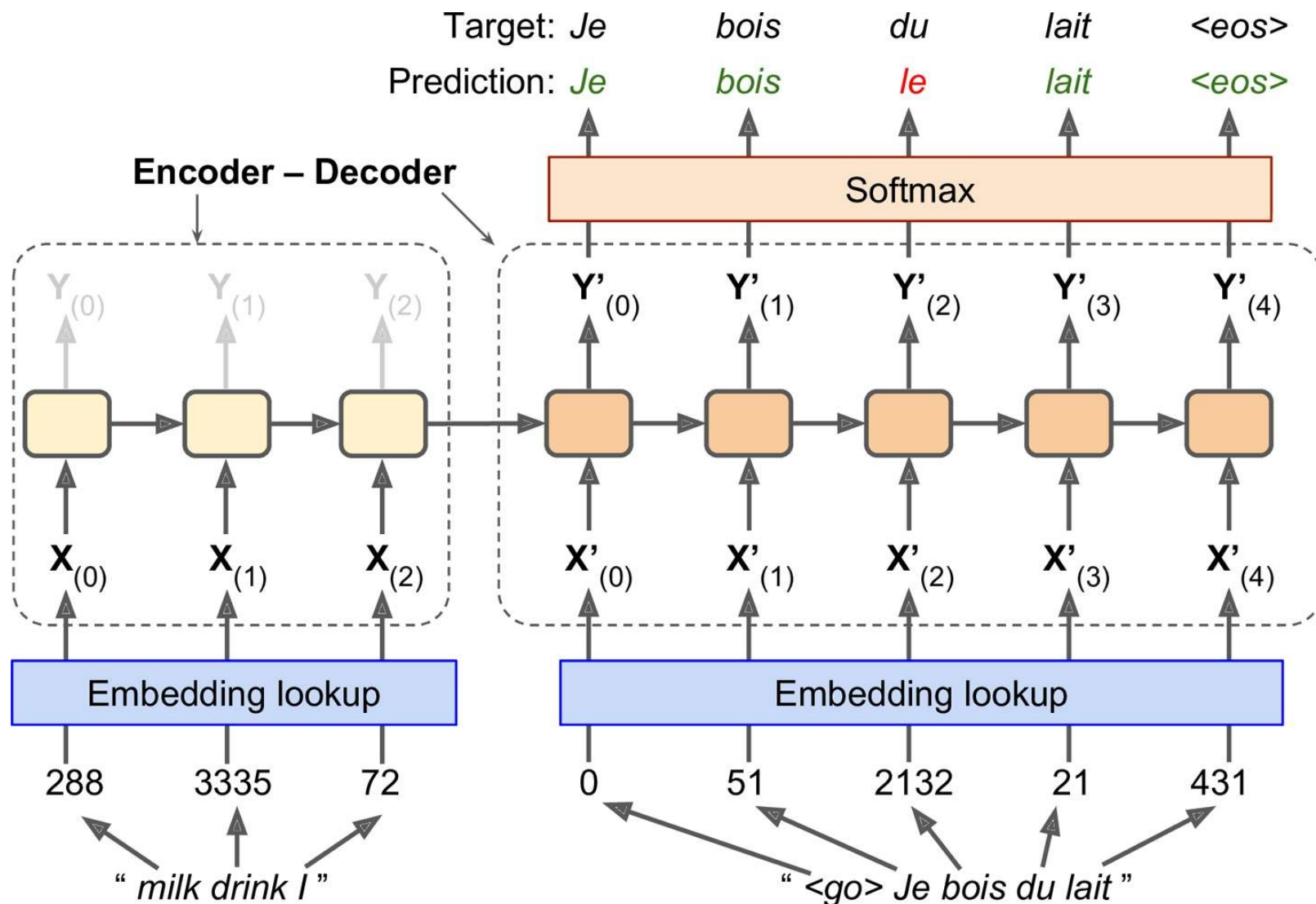
Figure 14-15. A simple machine translation model
