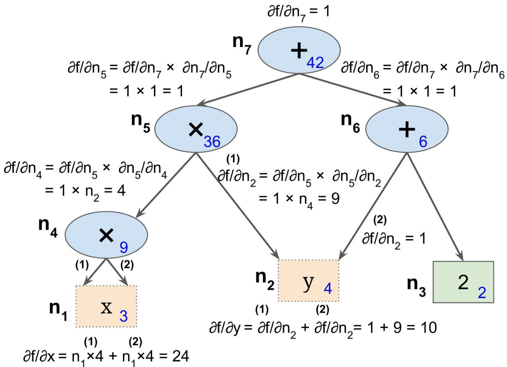
Figure D-3. Reverse-mode autodiff
