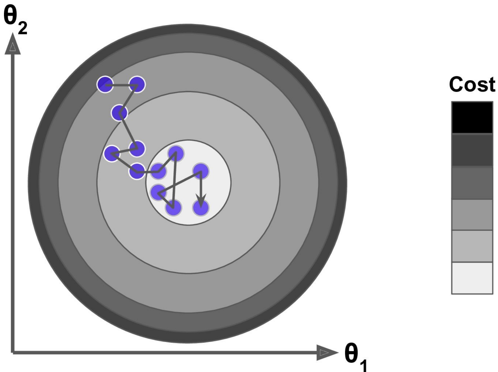
Figure 4-9. Stochastic Gradient Descent
