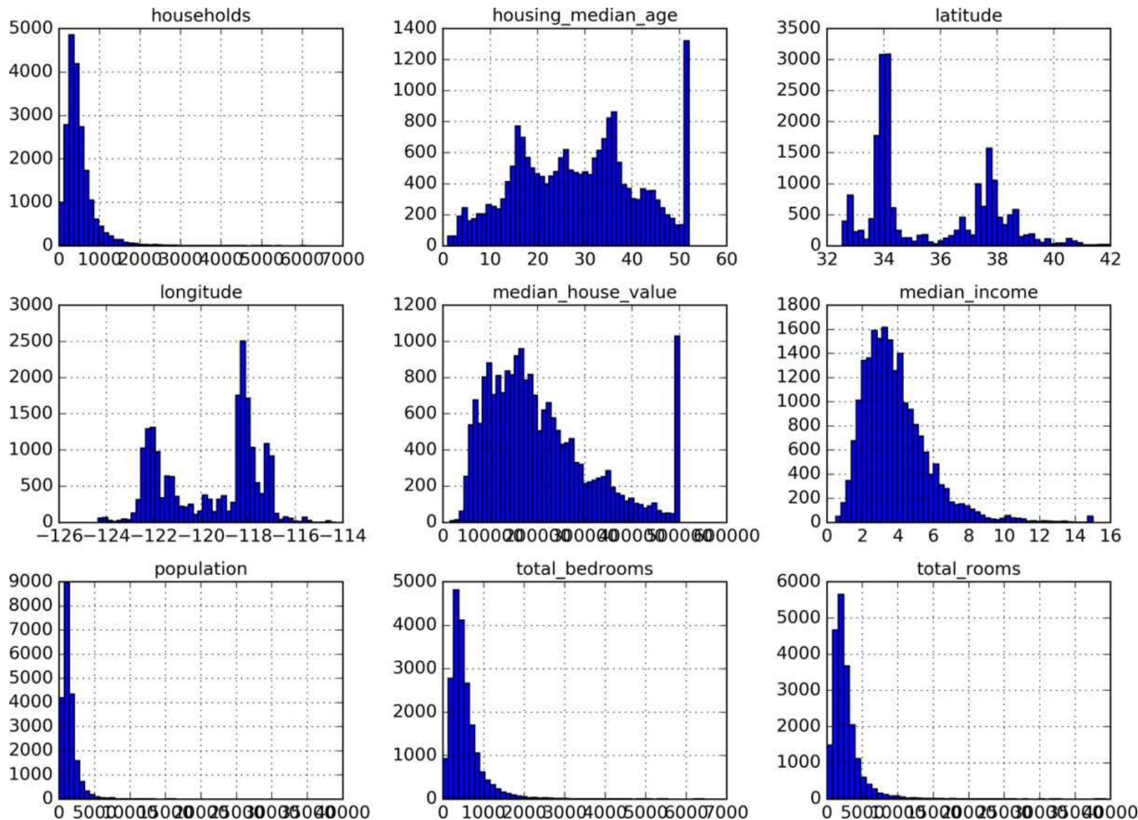
Figure 2-8. A histogram for each numerical attribute
