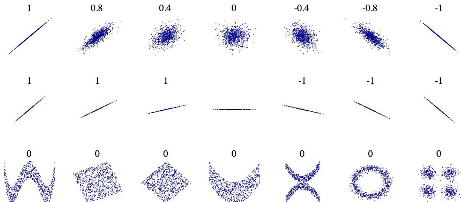
Figure 2-14. Standard correlation coefficient of various datasets (source: Wikipedia; public domain image)
