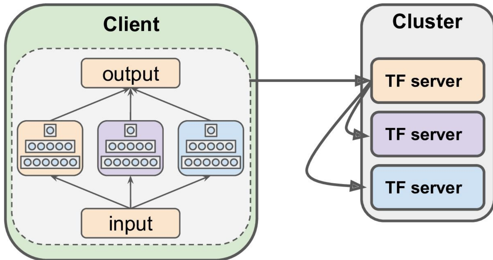
Figure 12-12. In-graph replication
