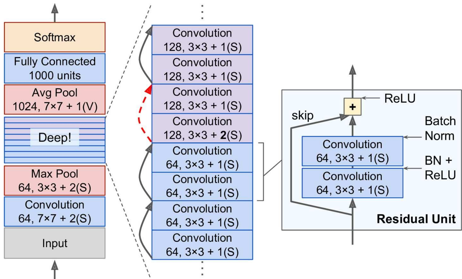
Figure 13-14. ResNet architecture
