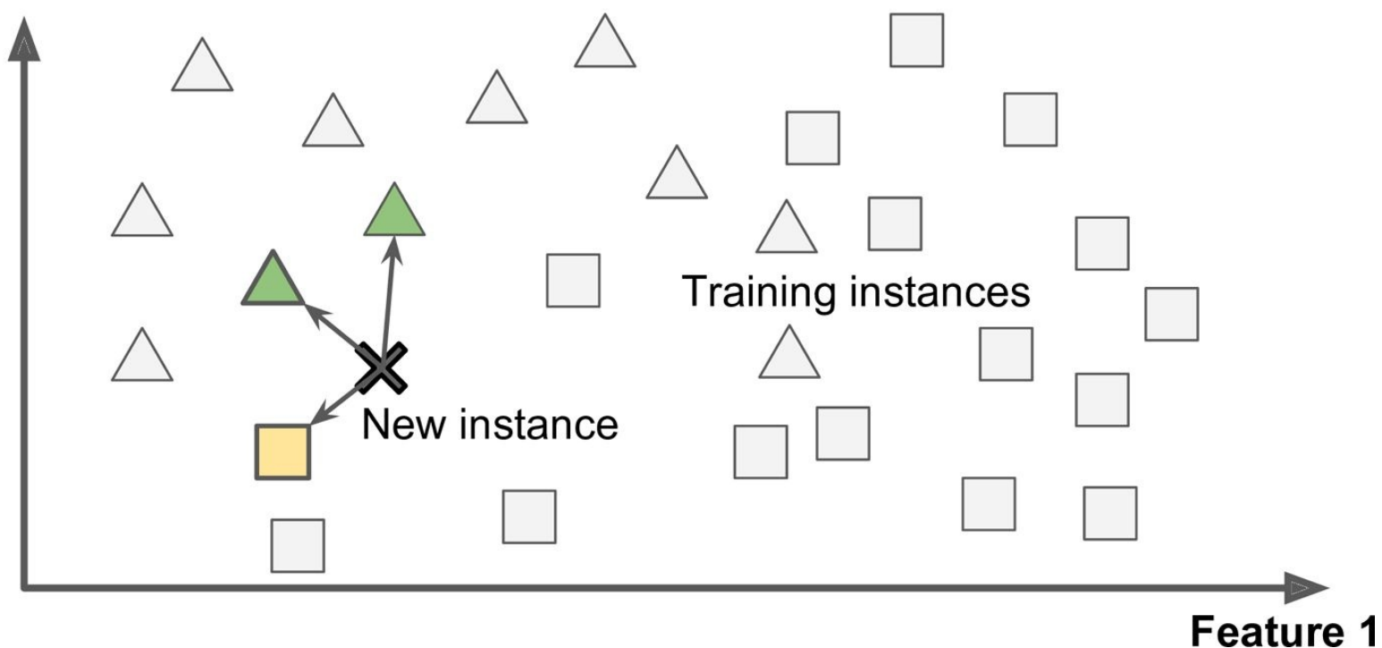
Figure 1-15. Instance-based learning
