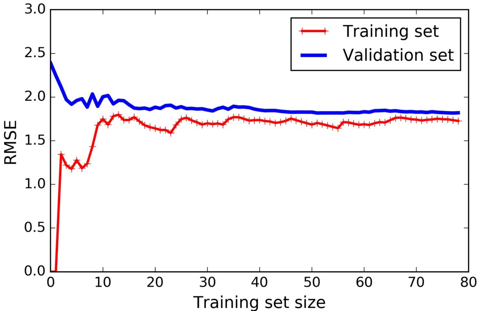
Figure 4-15. Learning curves
