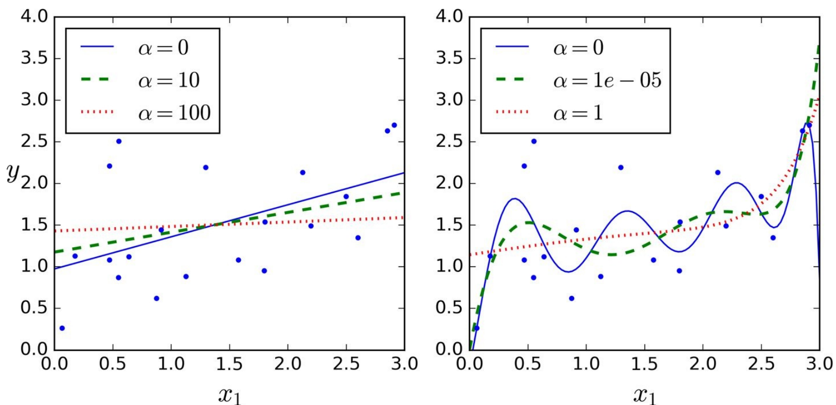
Figure 4-17. Ridge Regression
