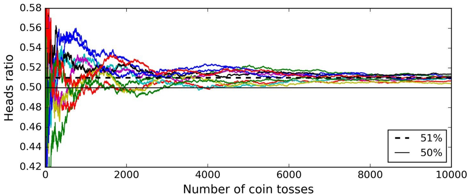
Figure 7-3. The law of large numbers
