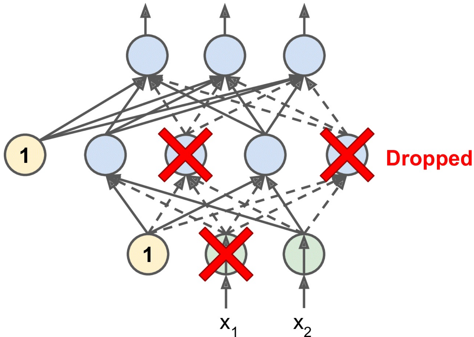
Figure 11-9. Dropout regularization
