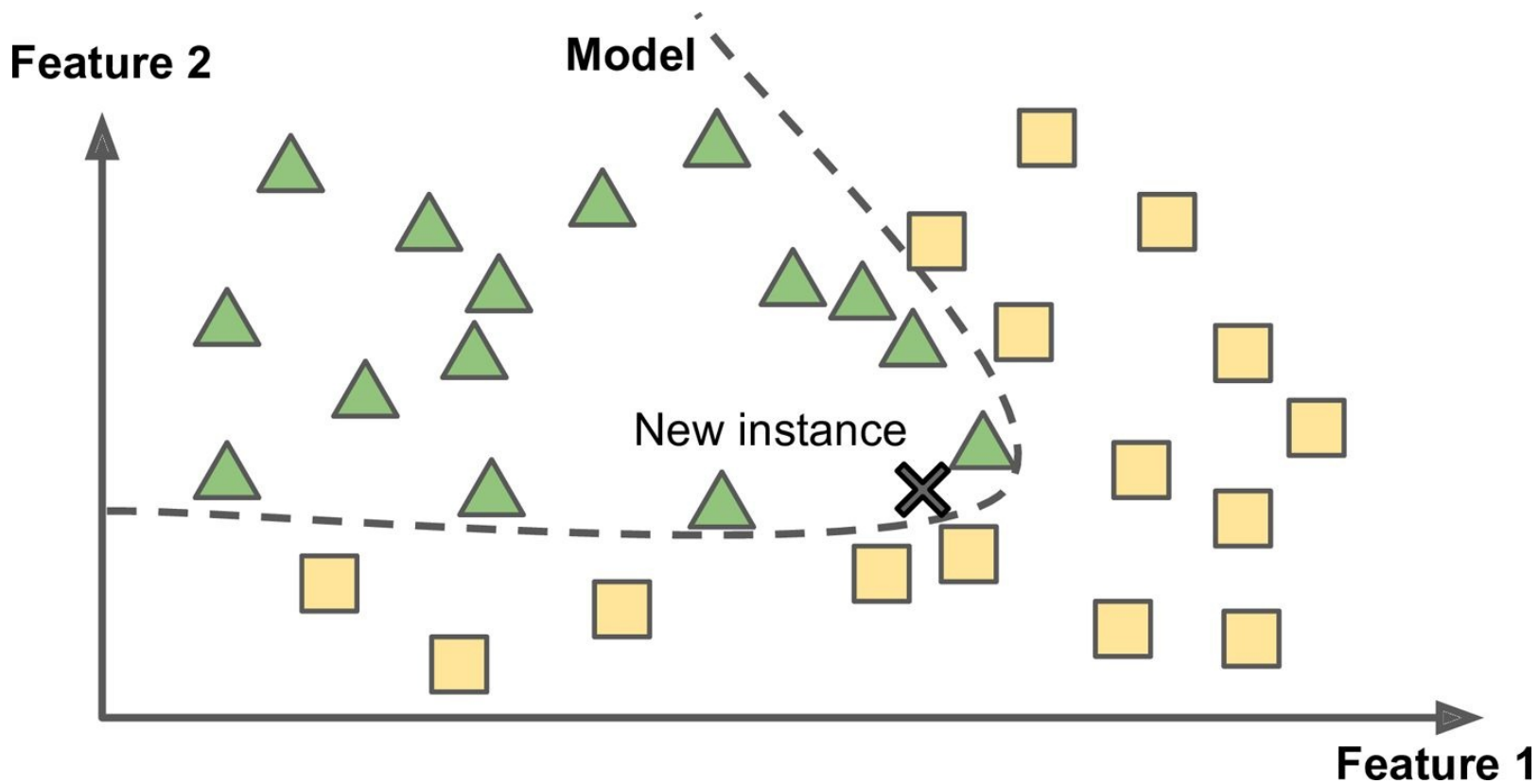
Figure 1-16. Model-based learning
