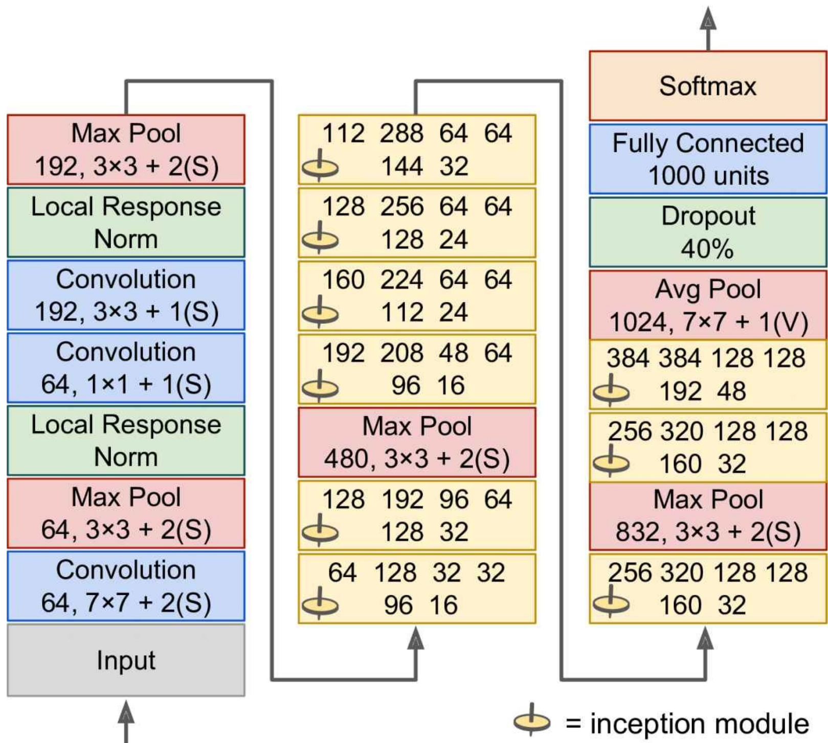
Figure 13-11. GoogLeNet architecture
