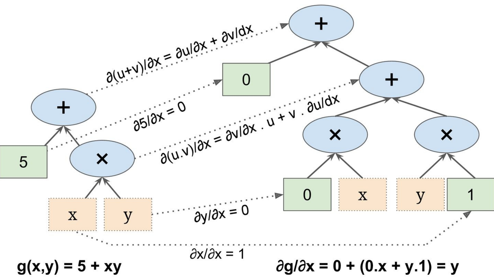
Figure D-1. Symbolic differentiation
