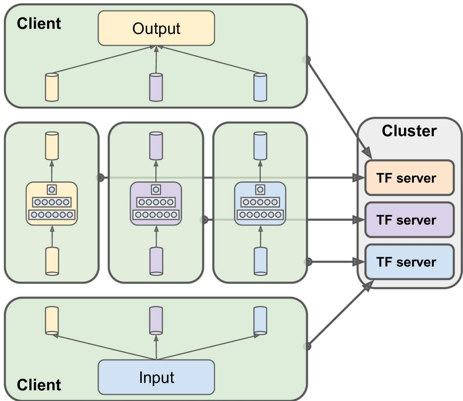
Figure 12-13. Between-graph replication
