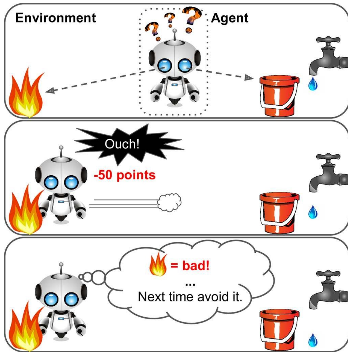
Figure 1-12. Reinforcement Learning
