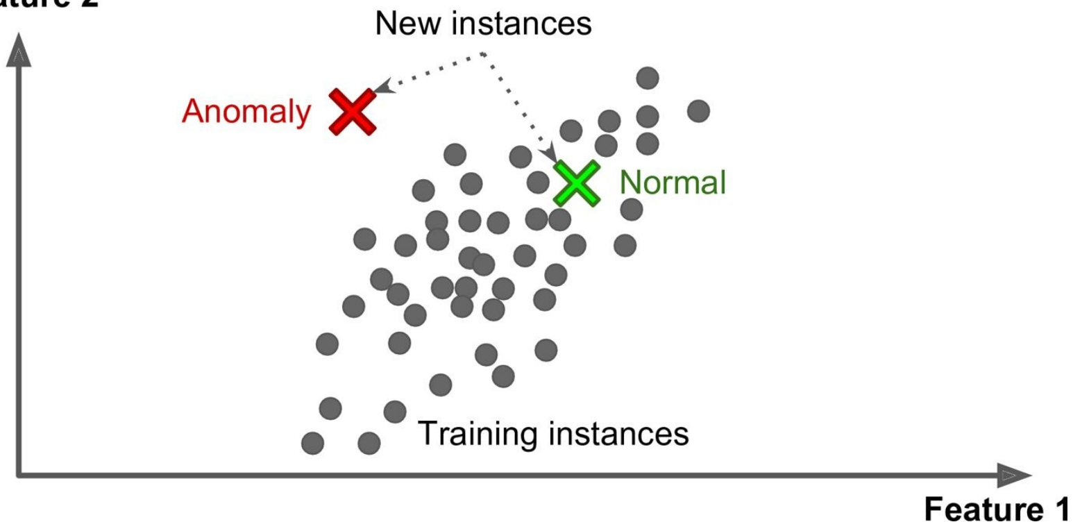
Figure 1-10. Anomaly detection
