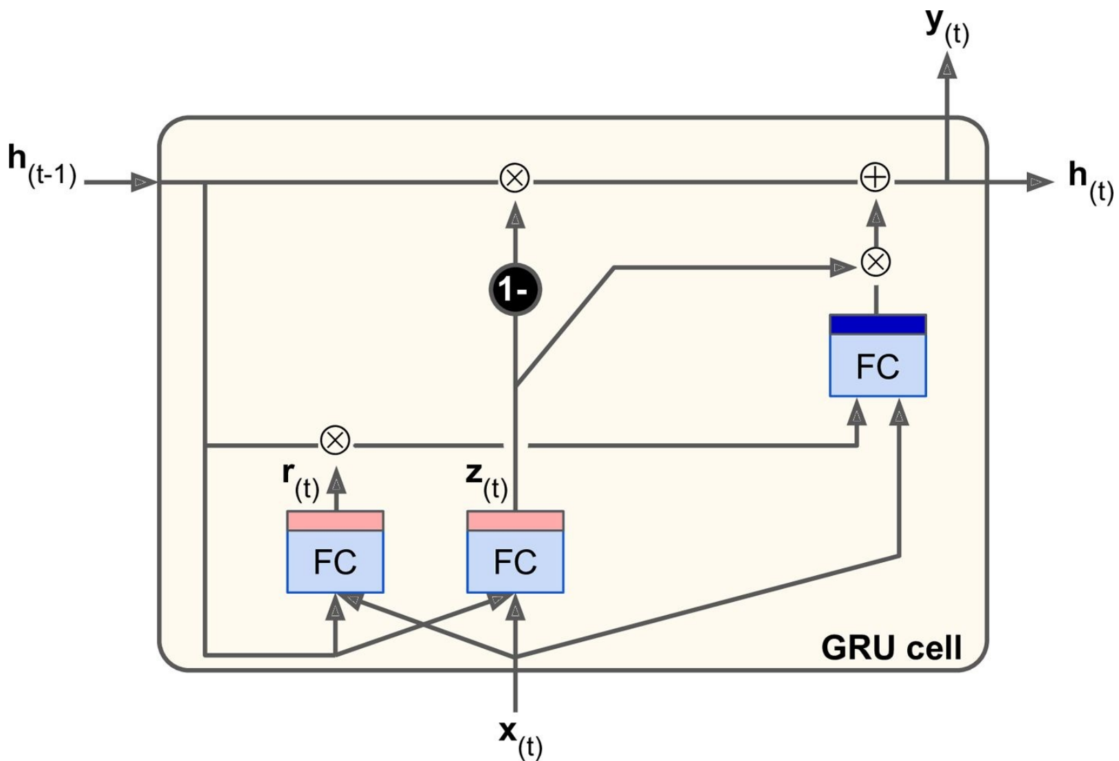
Figure 14-14. GRU cell
