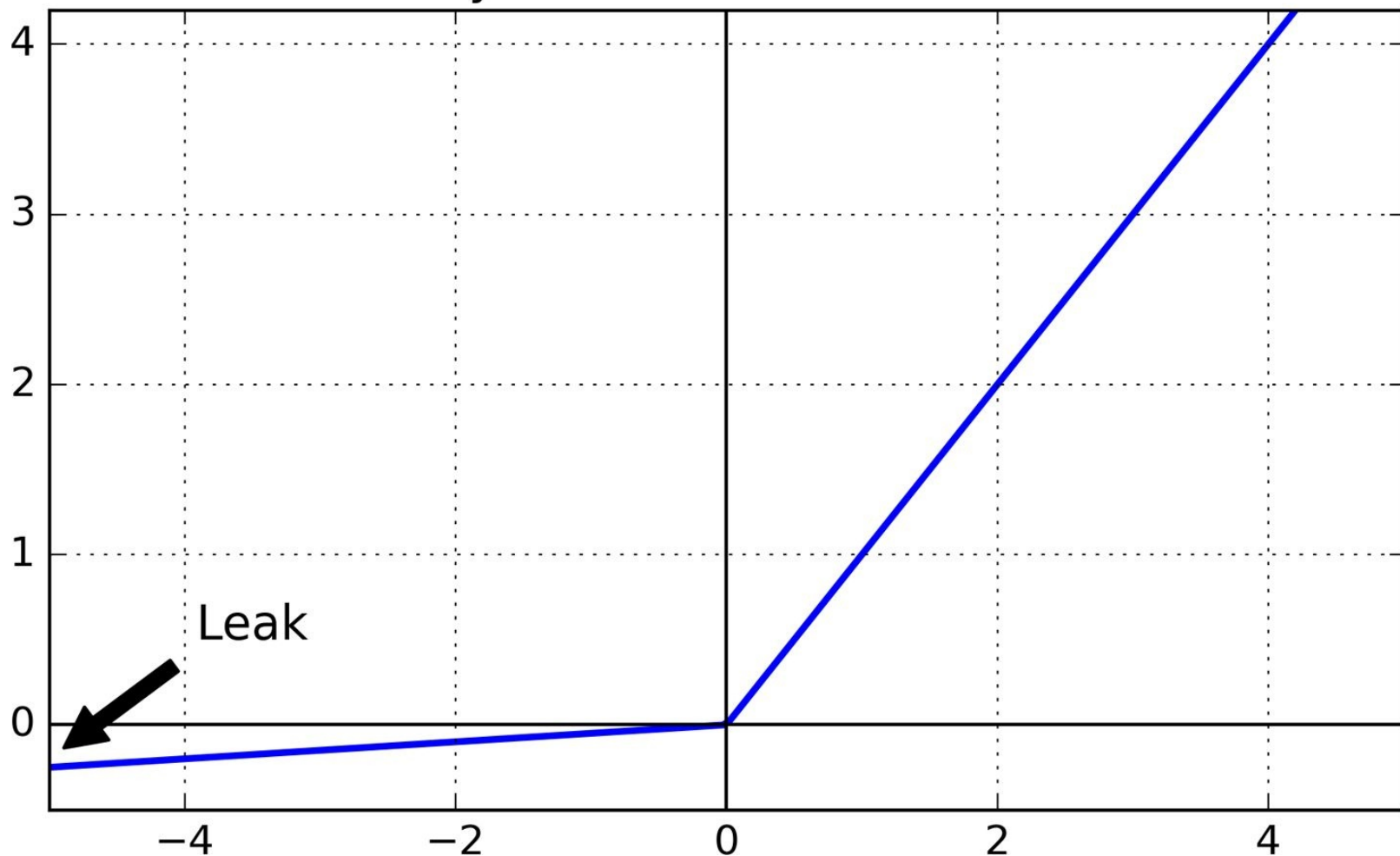
Figure 11-2. Leaky ReLU
