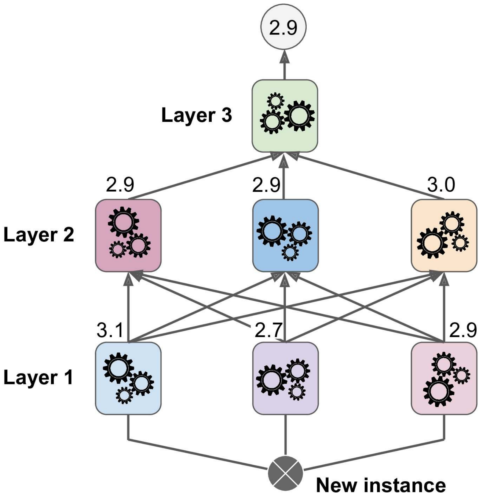
Figure 7-15. Predictions in a multilayer stacking ensemble
