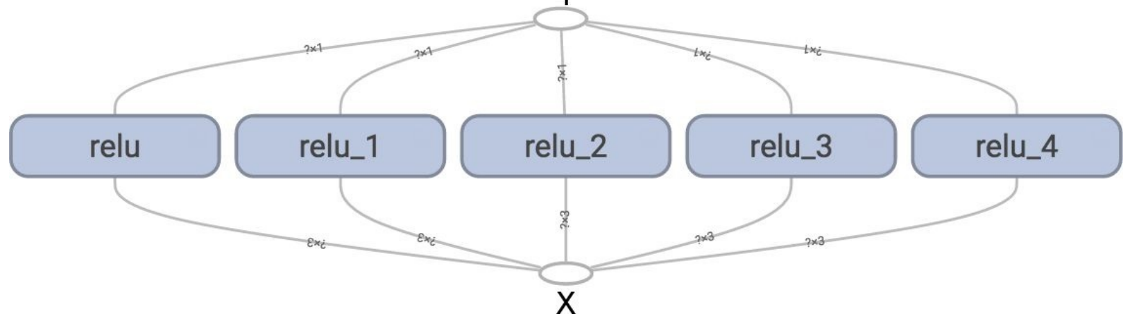
Figure 9-7. A clearer graph using name-scoped units
