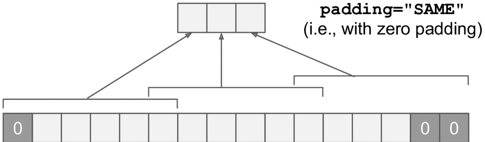
Figure 13-7. Padding options — input width: 13, filter width: 6, stride: 5
