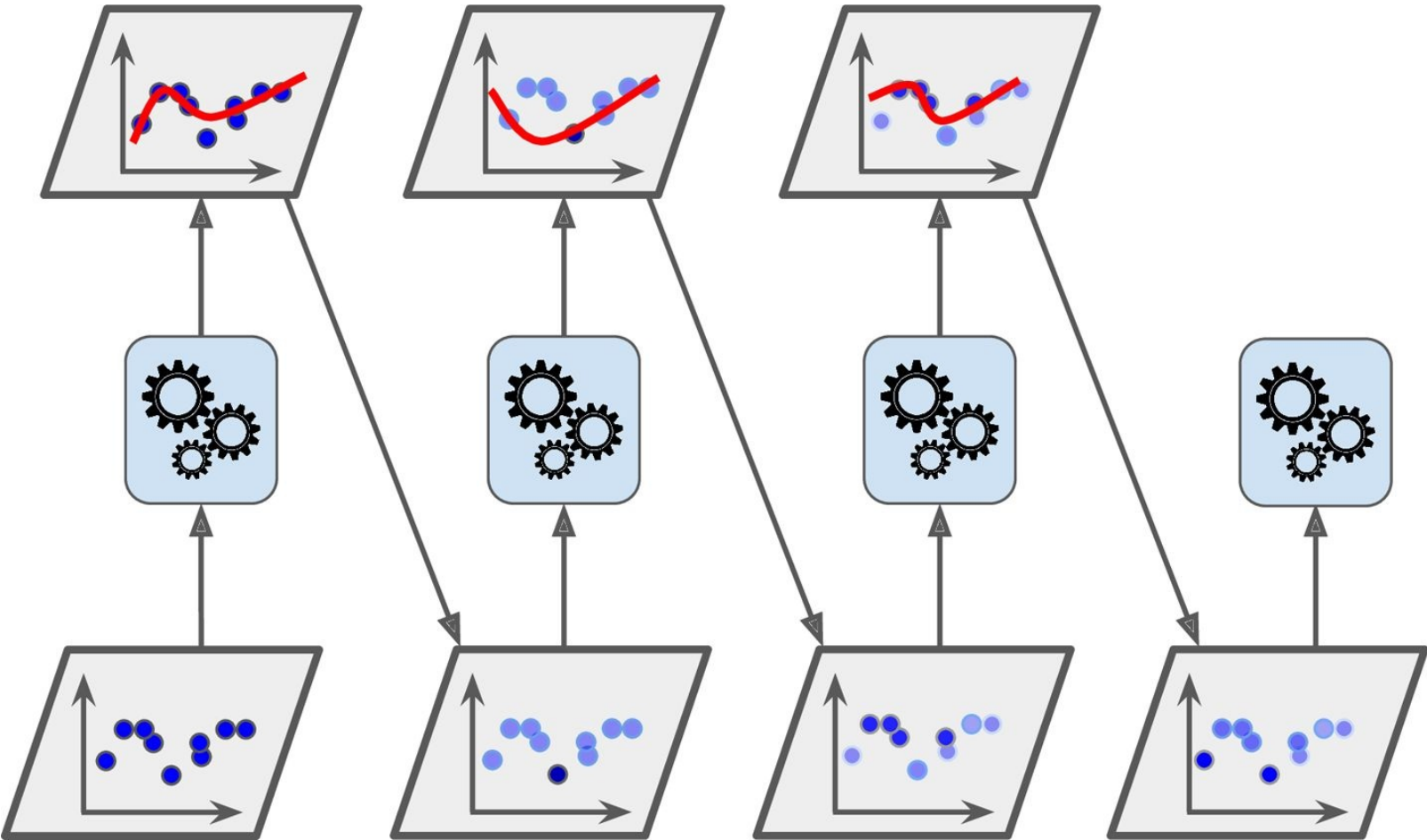
Figure 7-7. AdaBoost sequential training with instance weight updates
