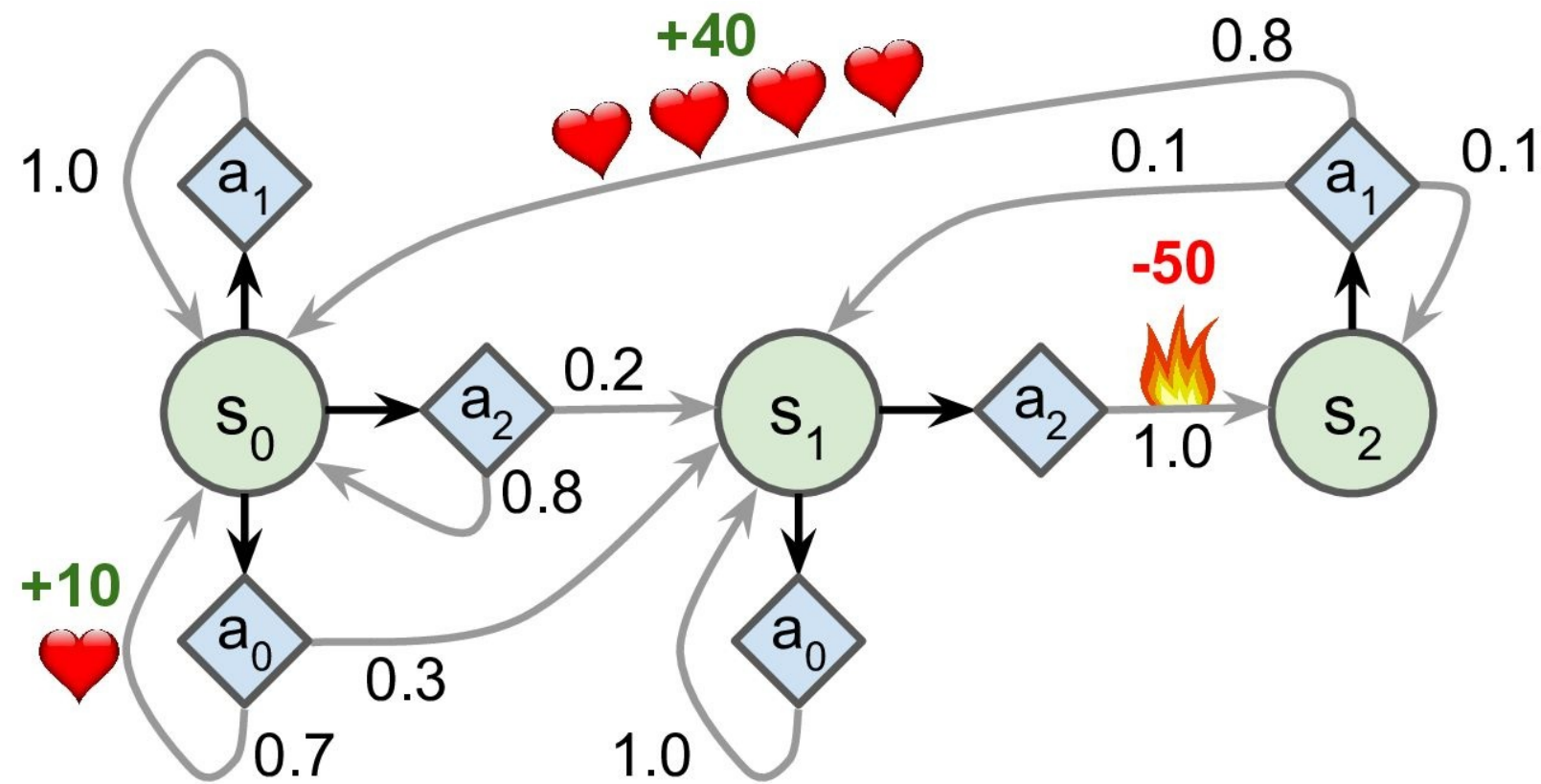
Figure 16-8. Example of a Markov decision process
