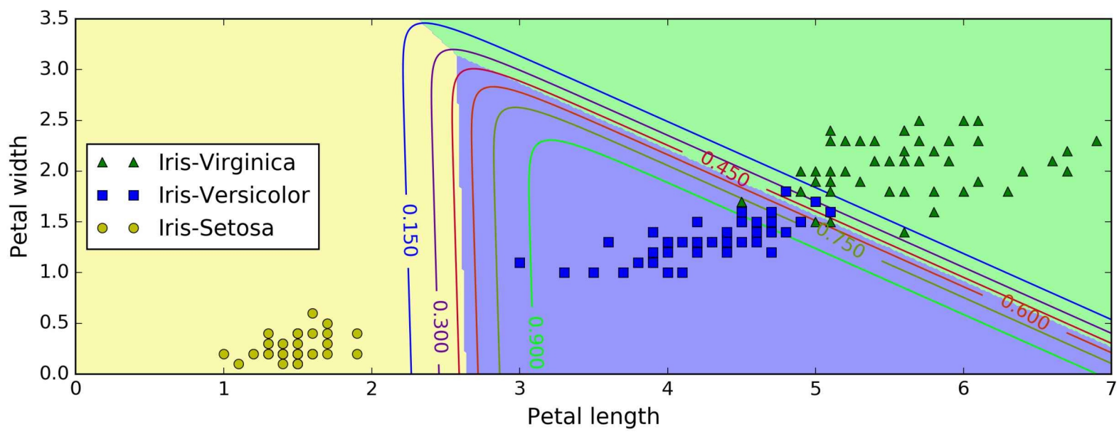
Figure 4-25. Softmax Regression decision boundaries
