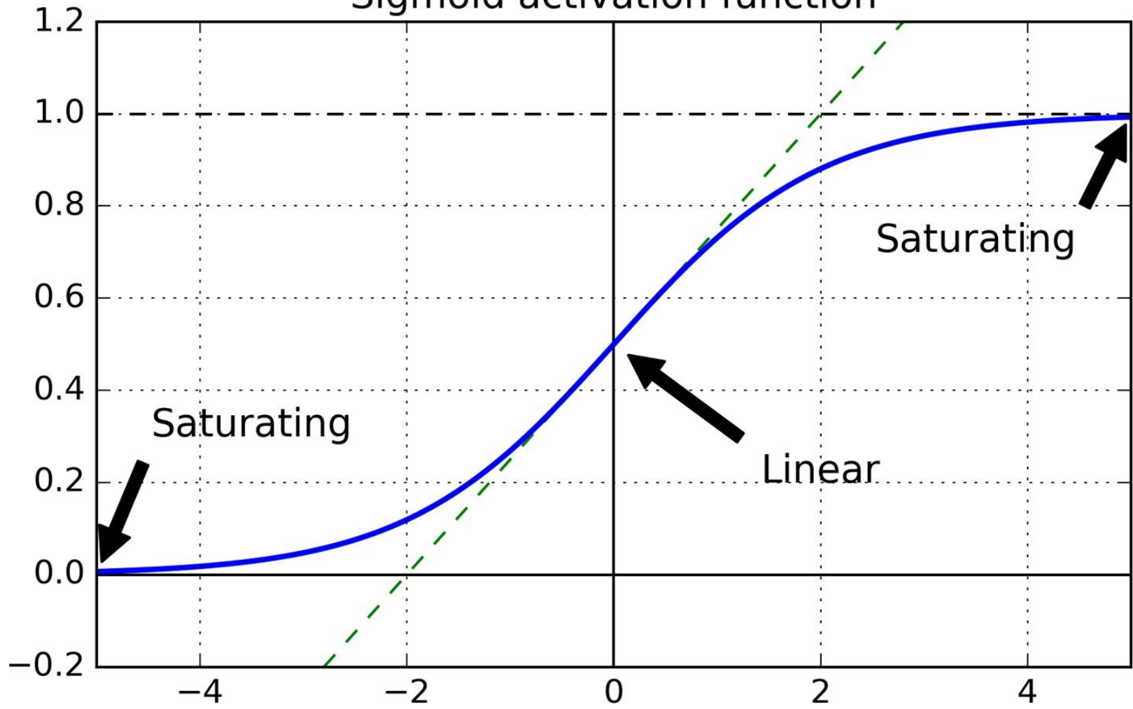
Figure 11-1. Logistic activation function saturation
