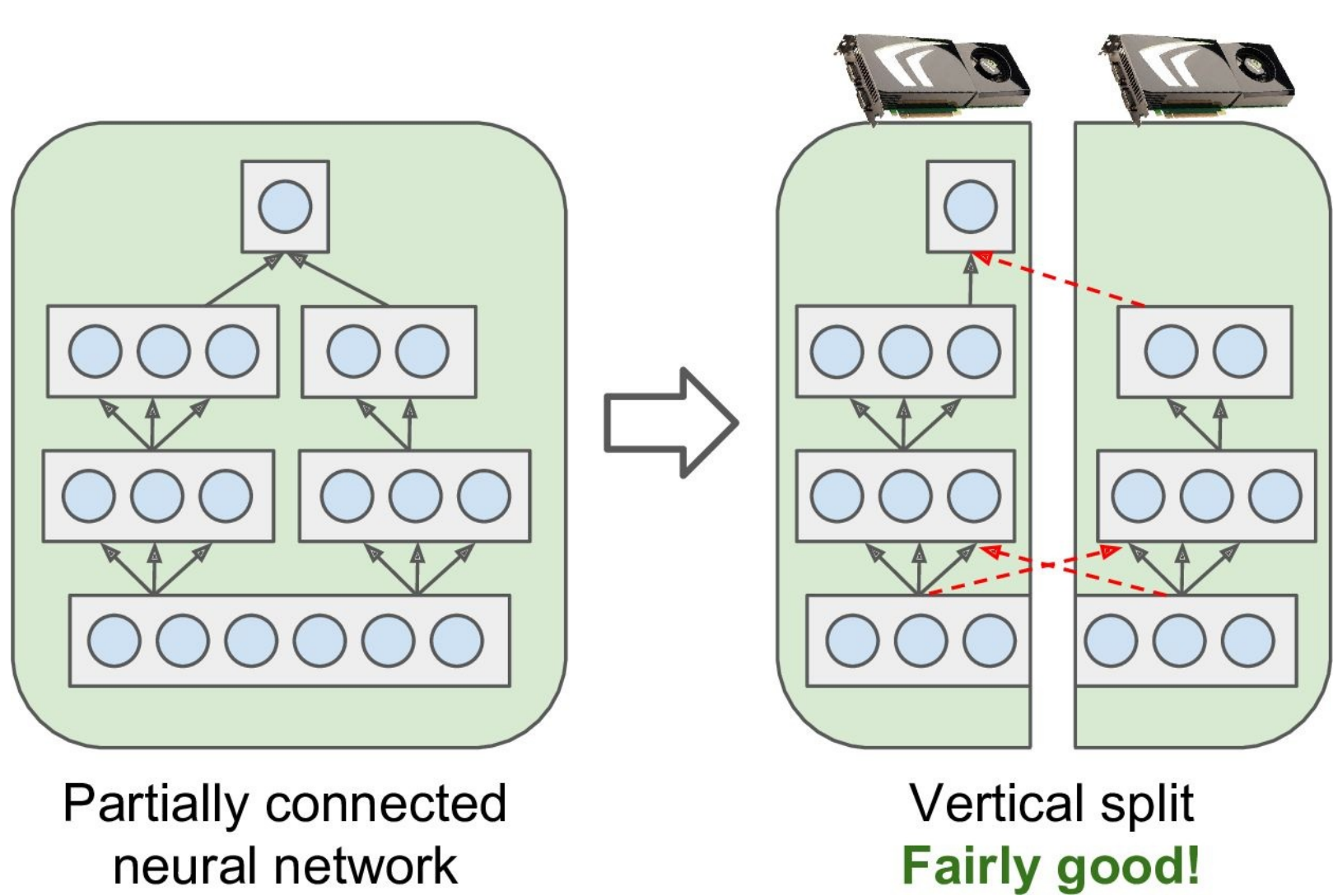
Figure 12-15. Splitting a partially connected neural network
