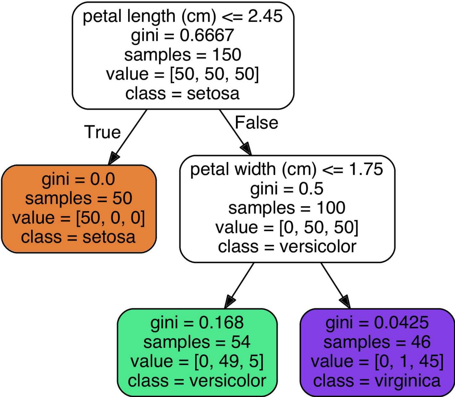
Figure 6-1. Iris Decision Tree
