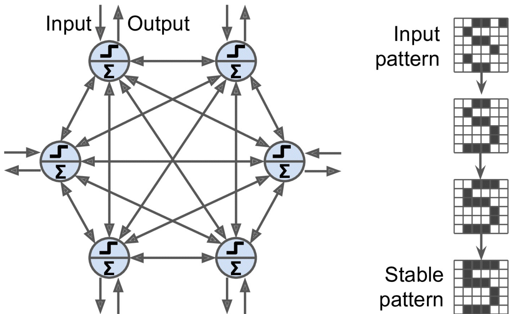
Figure E-1. Hopfield network
