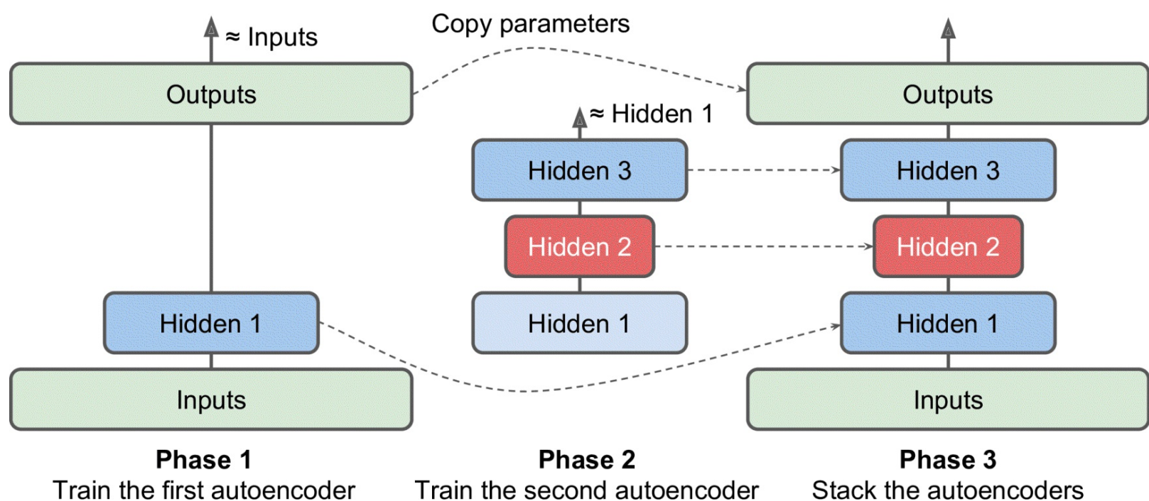
Figure 15-4. Training one autoencoder at a time
