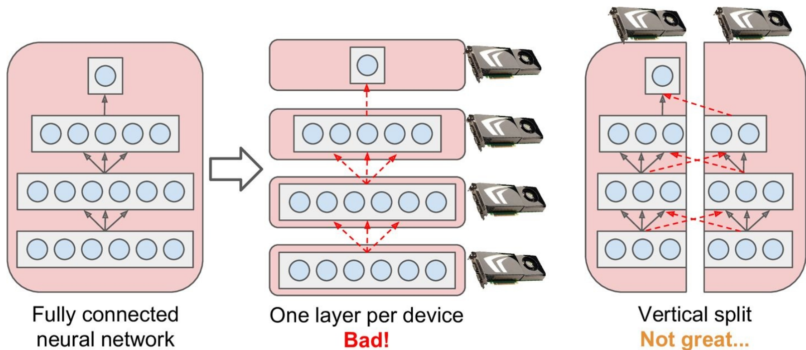
Figure 12-14. Splitting a fully connected neural network
