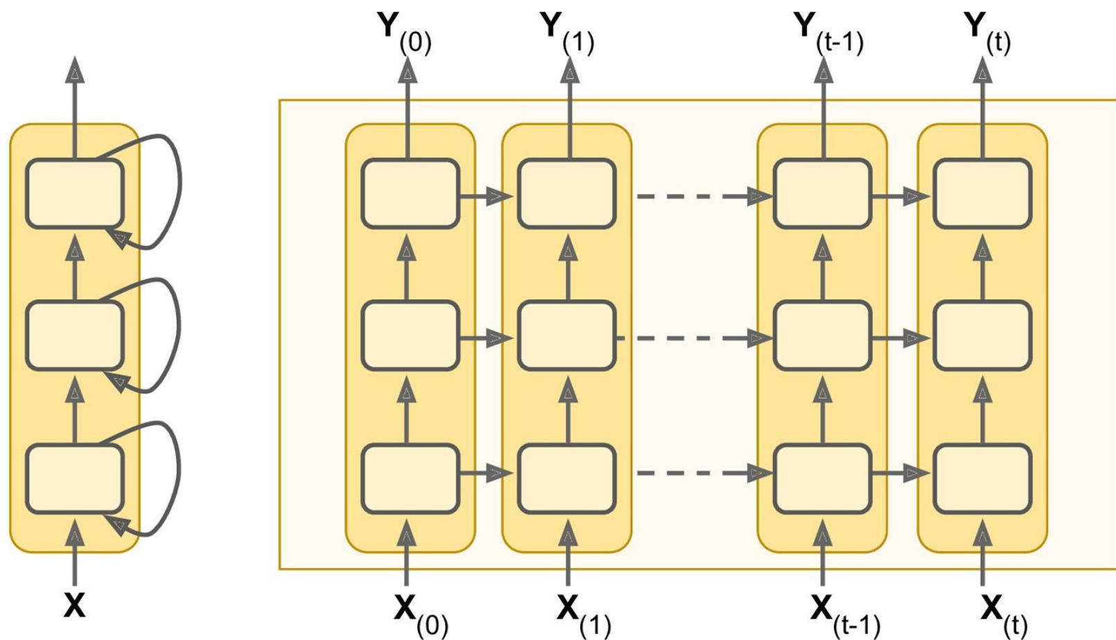
Figure 14-12. Deep RNN (left), unrolled through time (right)
