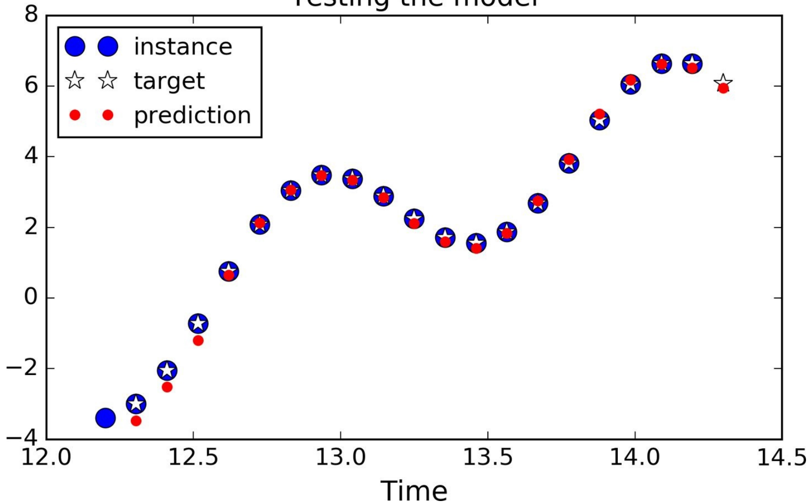
Figure 14-9. Time series prediction
