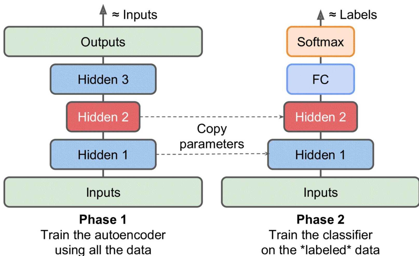
Figure 15-8. Unsupervised pretraining using autoencoders
