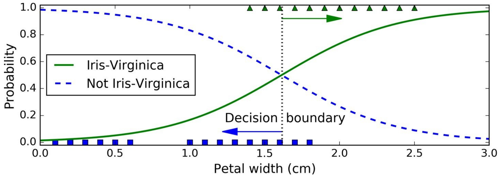
Figure 4-23. Estimated probabilities and decision boundary
