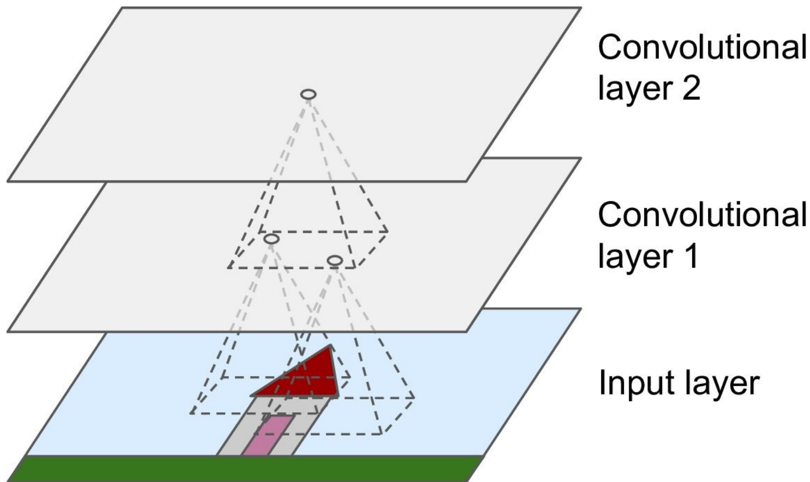
Figure 13-2. CNN layers with rectangular local receptive fields
