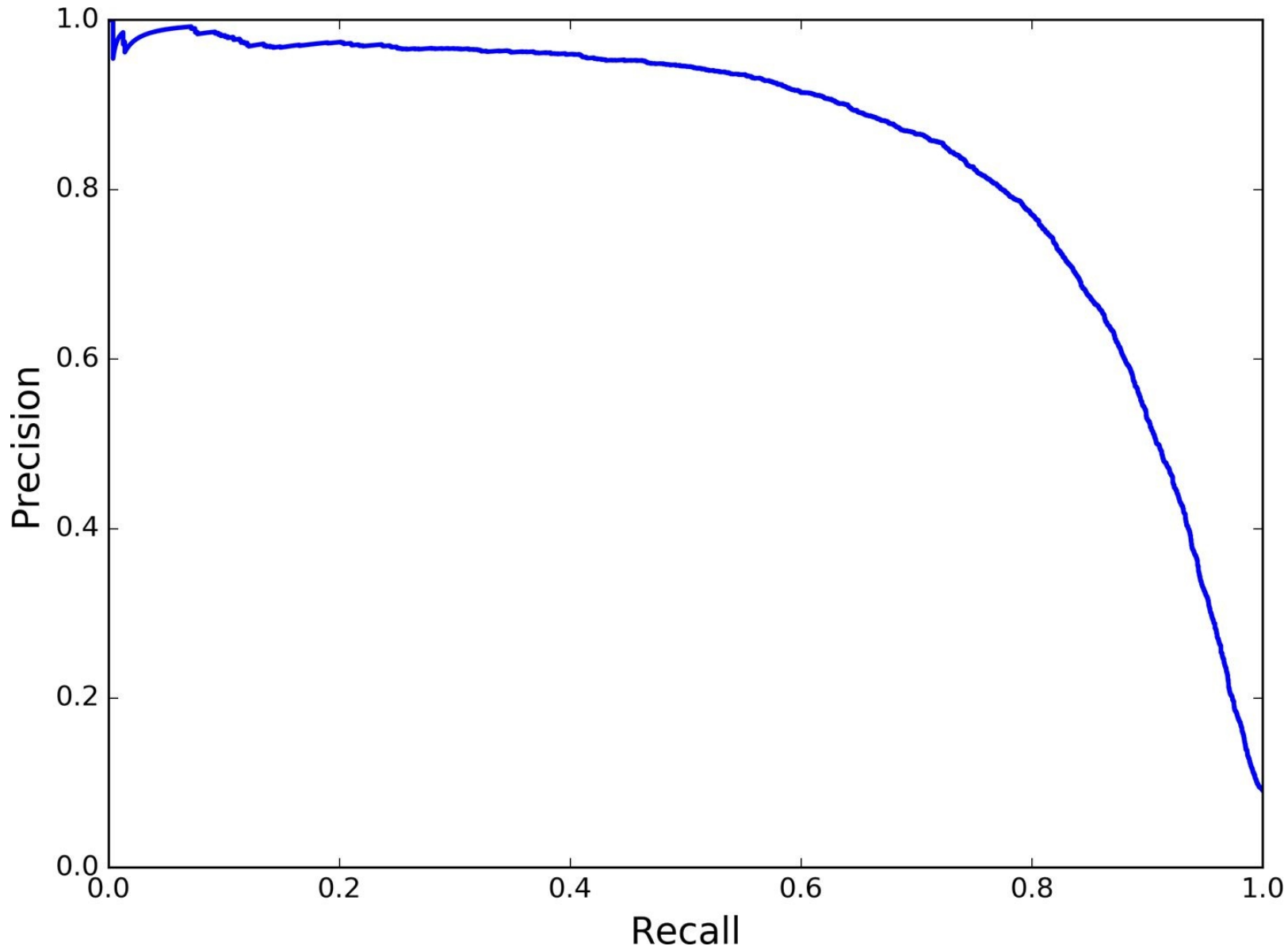
Figure 3-5. Precision versus recall
