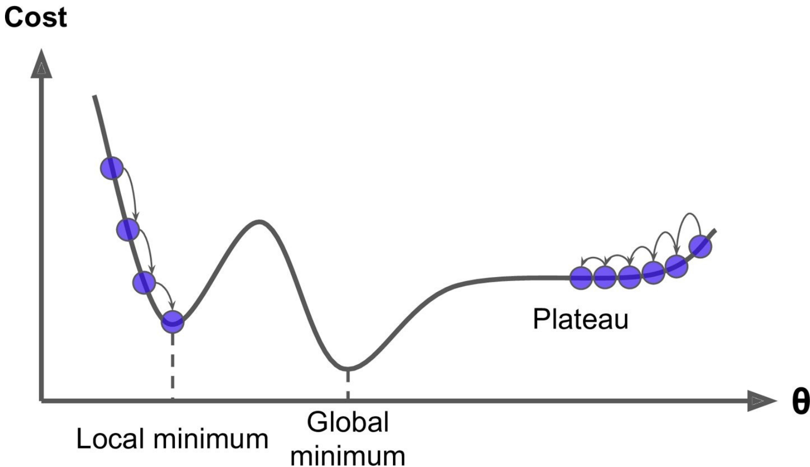
Figure 4-6. Gradient Descent pitfalls
