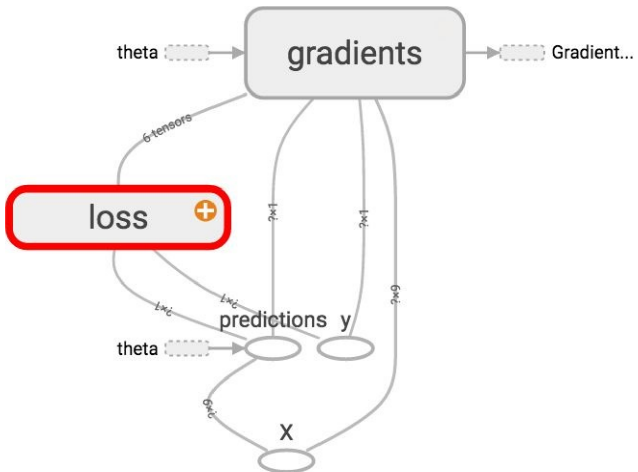
Figure 9-5. A collapsed namespace in TensorBoard
