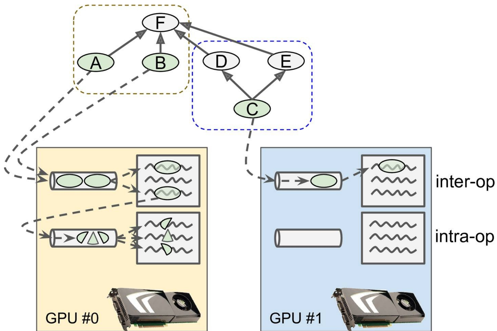
Figure 12-5. Parallelized execution of a TensorFlow graph
