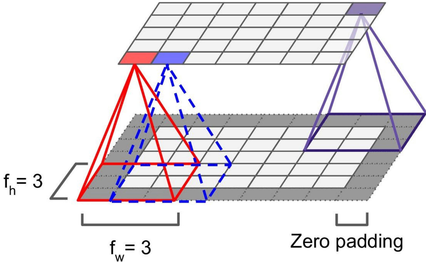
Figure 13-3. Connections between layers and zero padding
