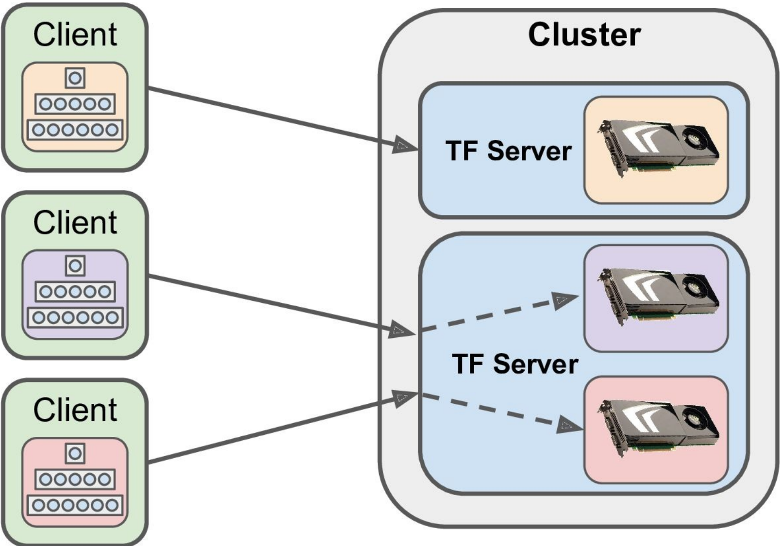
Figure 12-11. Training one neural network per device
