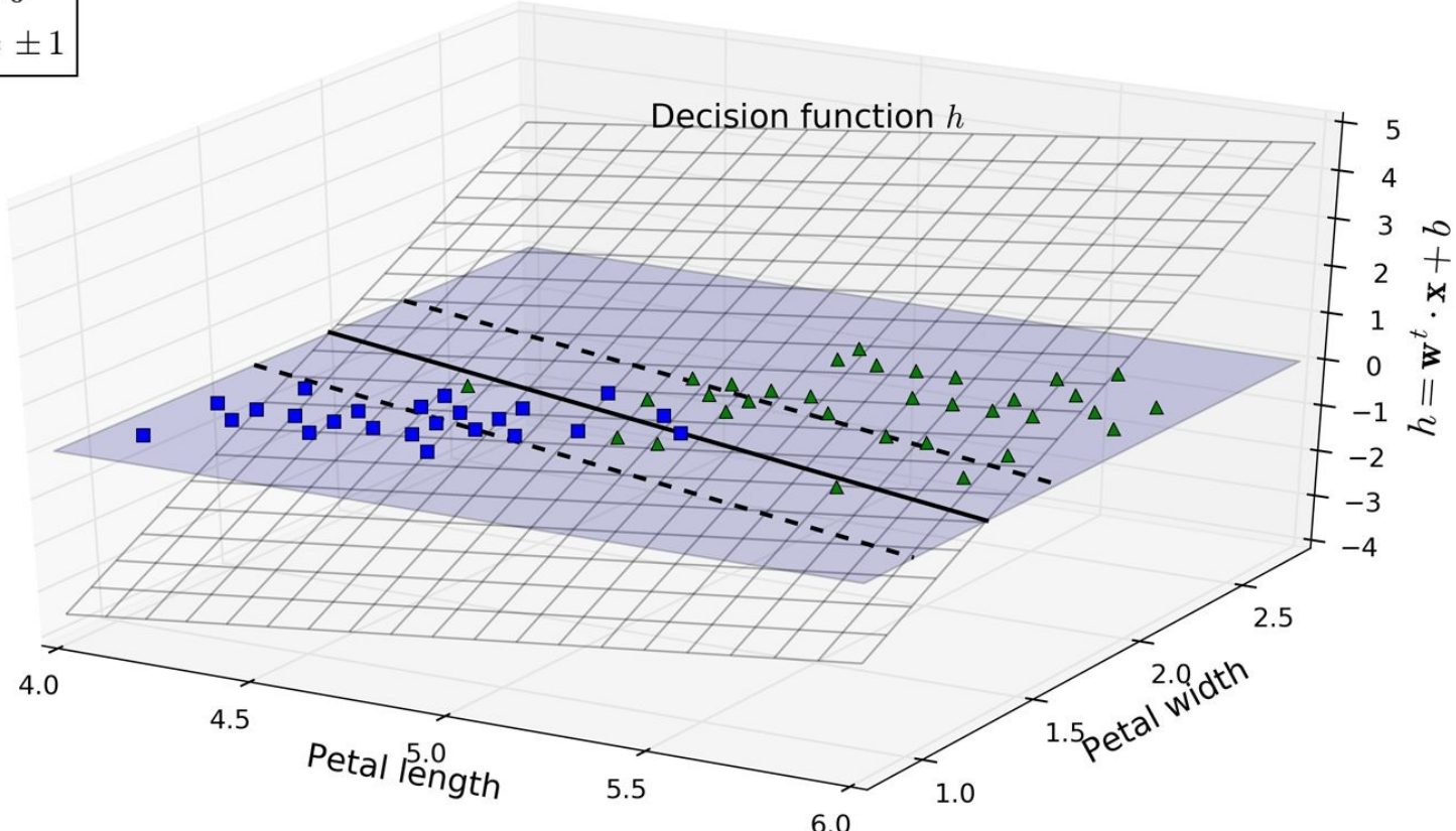
Figure 5-12. Decision function for the iris dataset
