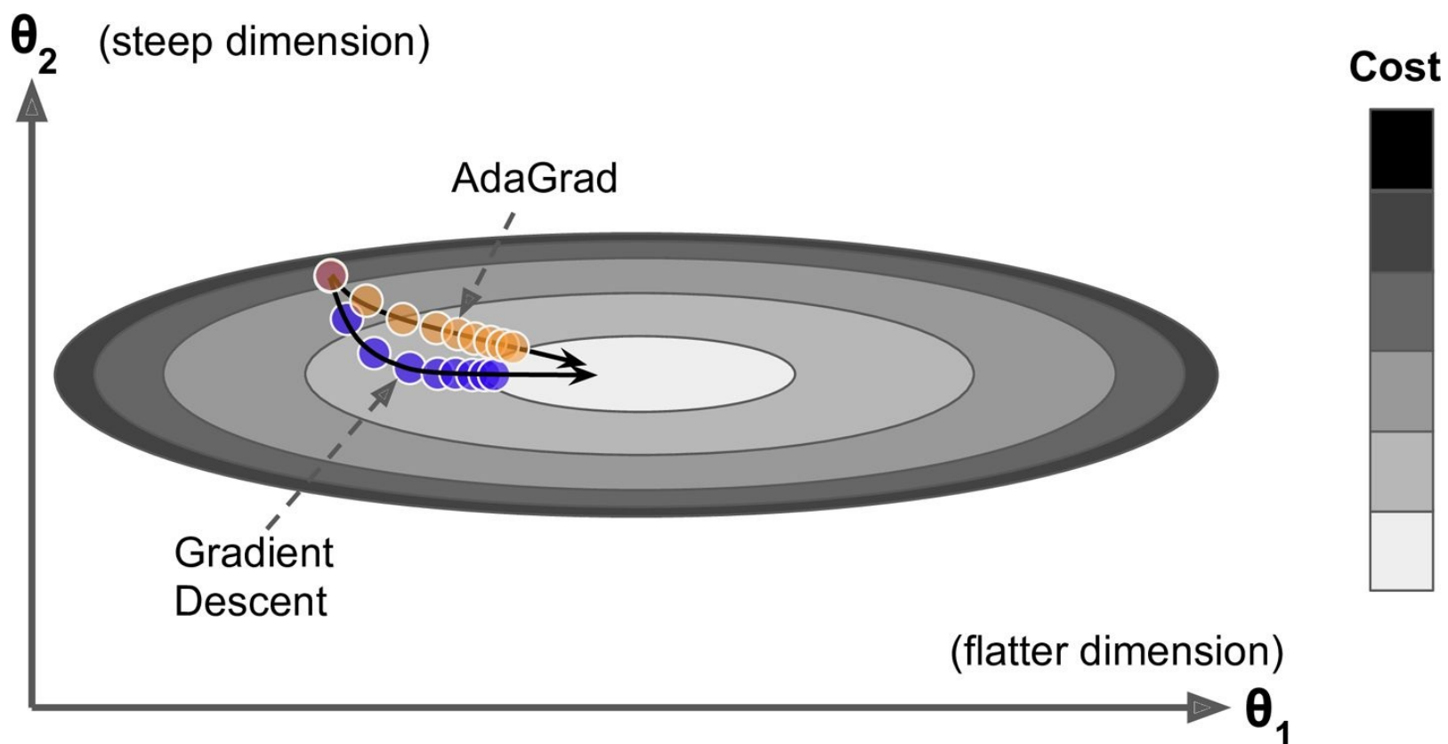
Figure 11-7. AdaGrad versus Gradient Descent
