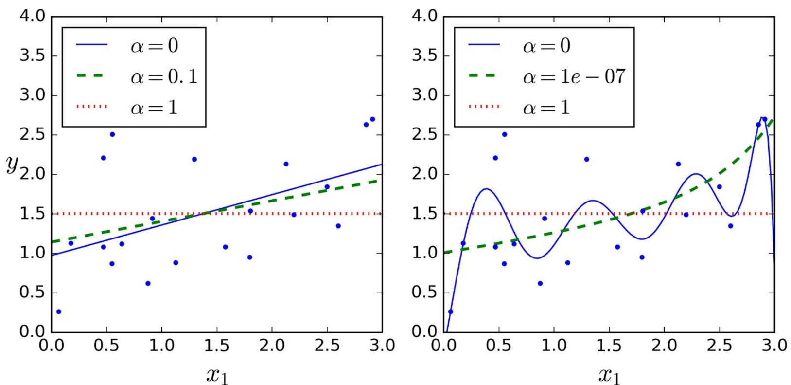
Figure 4-18. Lasso Regression
