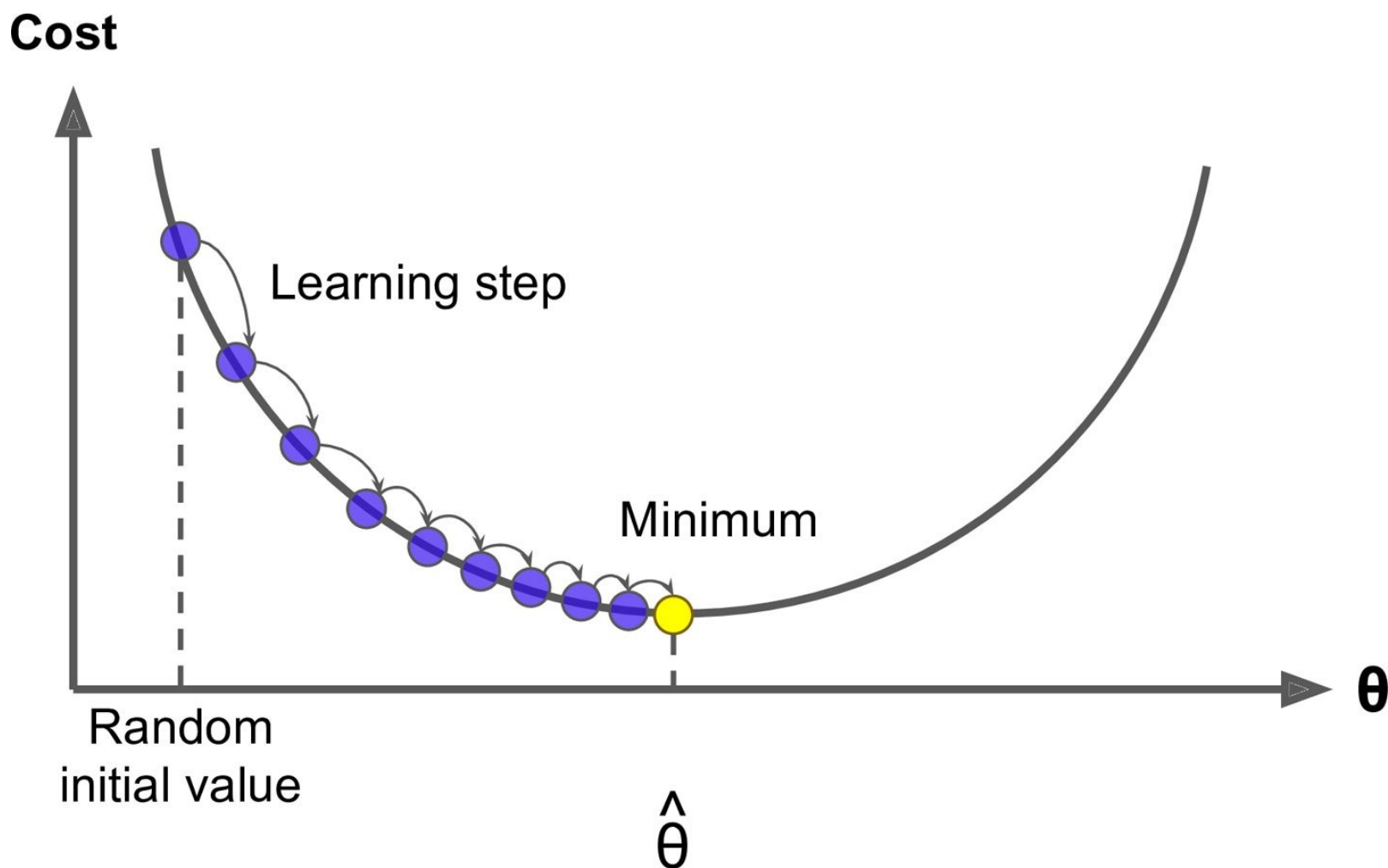
Figure 4-3. Gradient Descent
