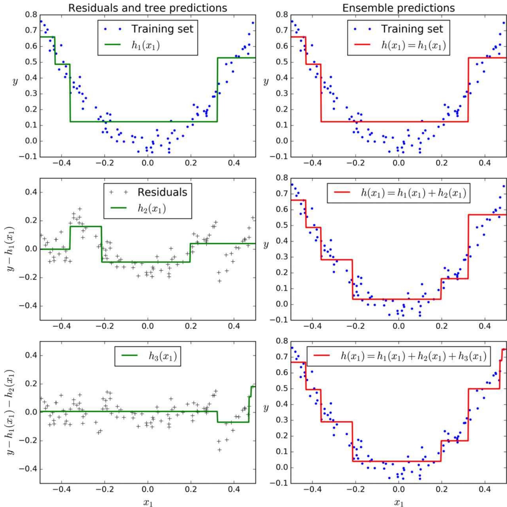
Figure 7-9. Gradient Boosting
