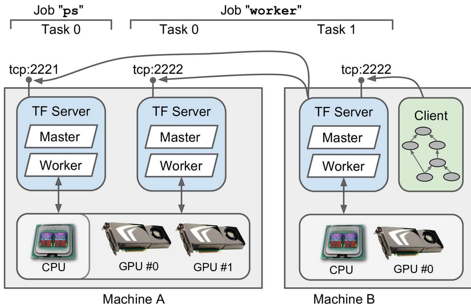
Figure 12-6. TensorFlow cluster
