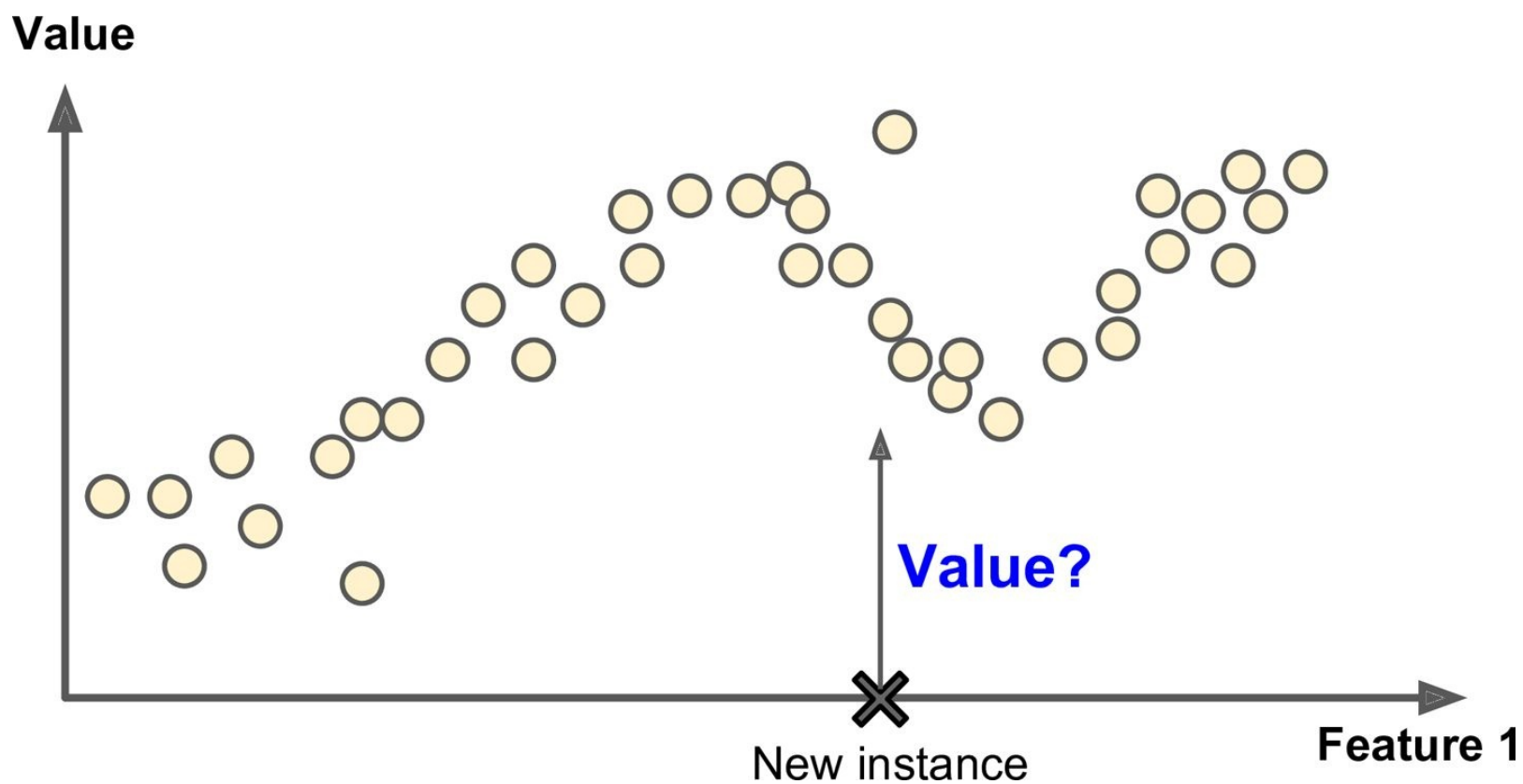
Figure 1-6. Regression
