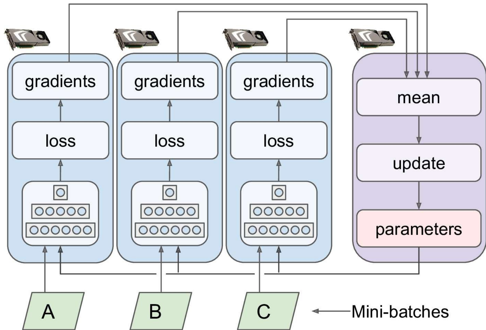
Figure 12-17. Data parallelism
