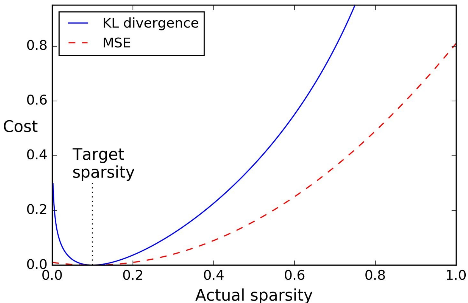
Figure 15-10. Sparsity loss
