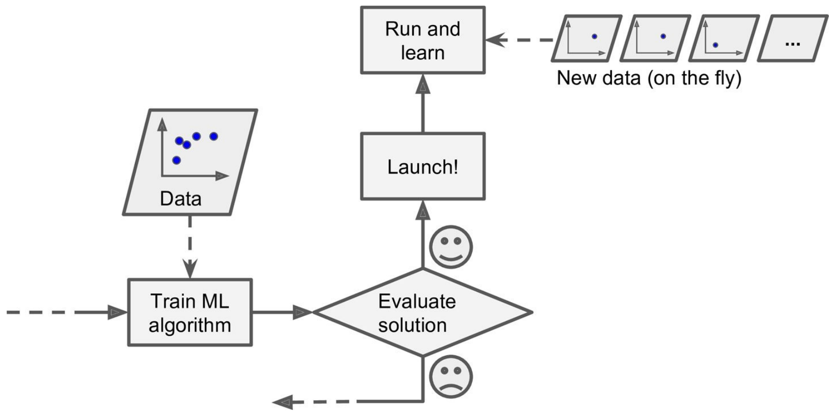
Figure 1-13. Online learning
