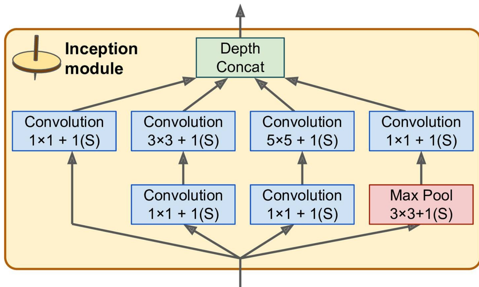
Figure 13-10. Inception module
