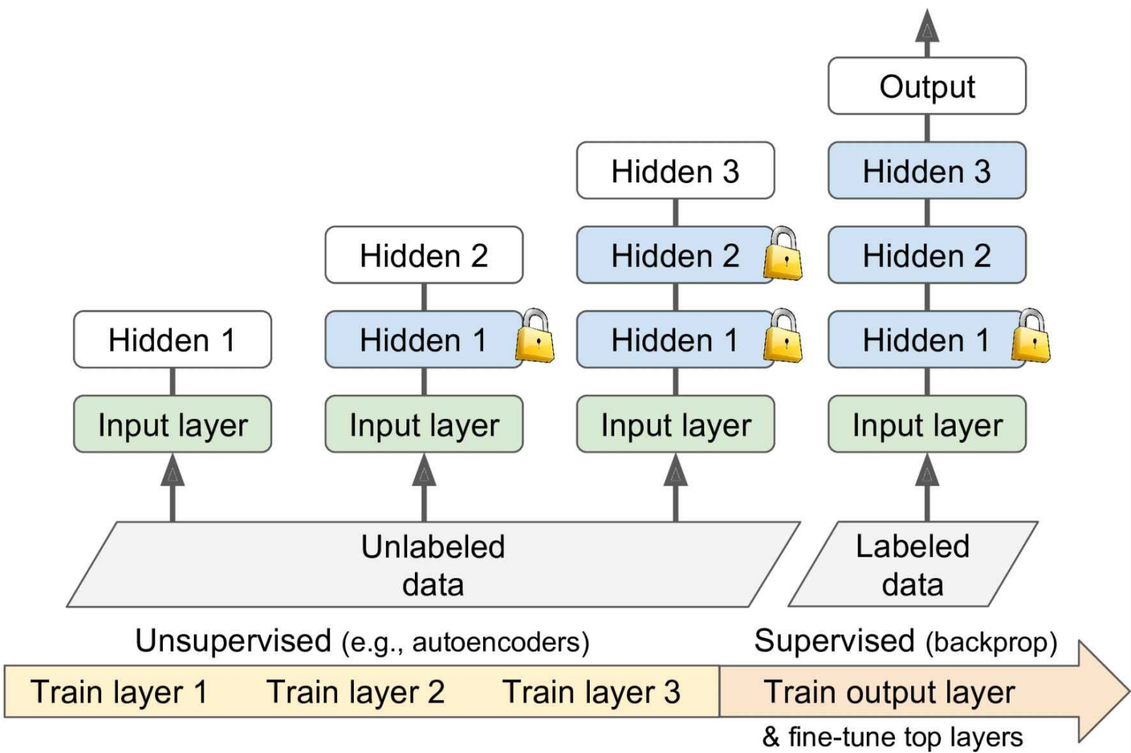
Figure 11-5. Unsupervised pretraining
