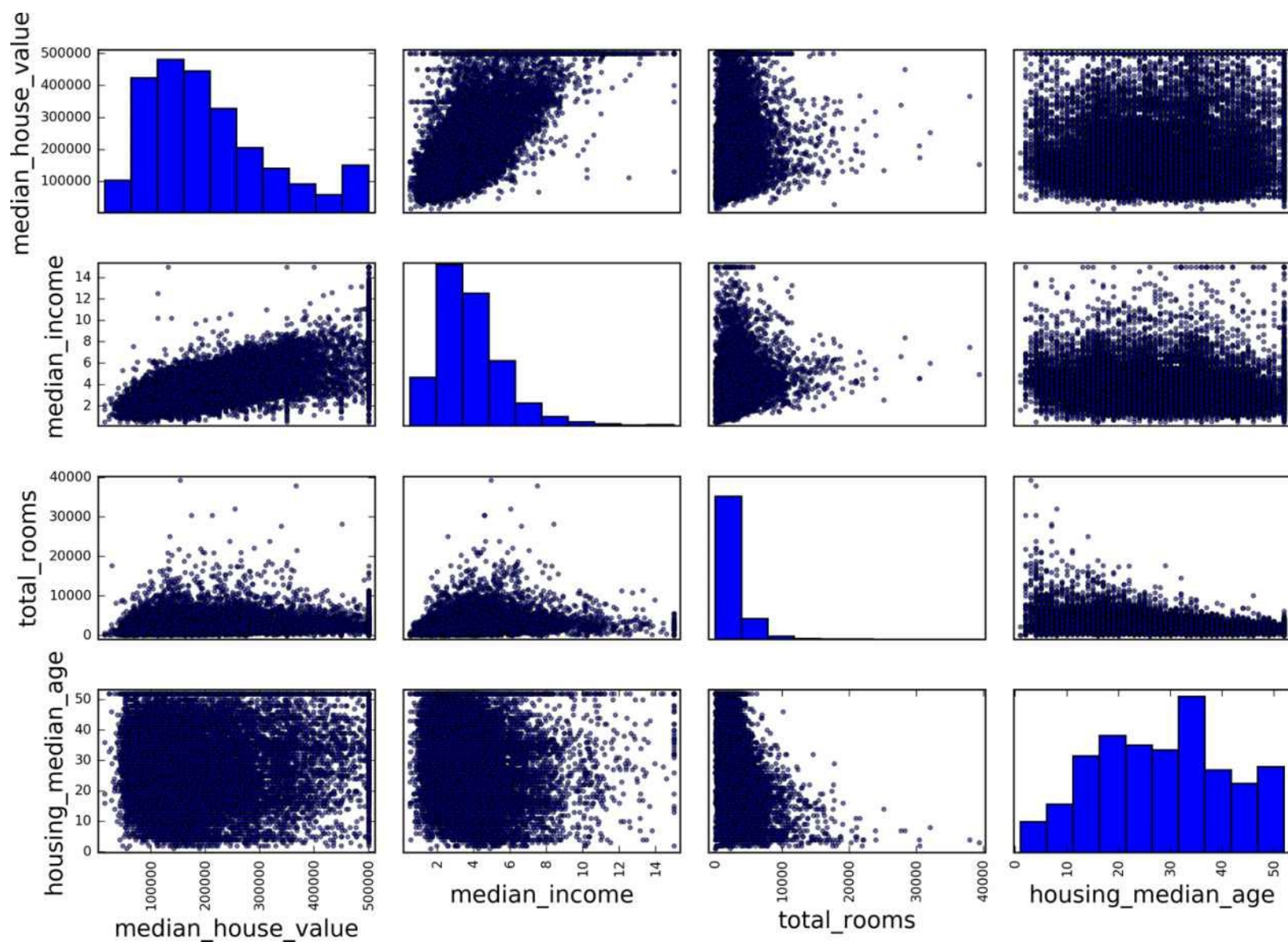
Figure 2-15. Scatter matrix
