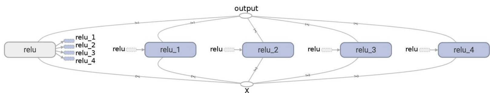
Figure 9-9. Five ReLUs sharing the threshold variable
