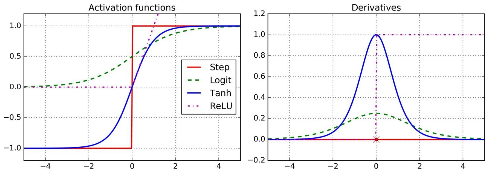
Figure 10-8. Activation functions and their derivatives
