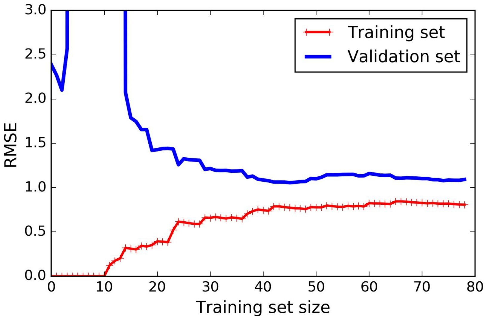
Figure 4-16. Learning curves for the polynomial model
