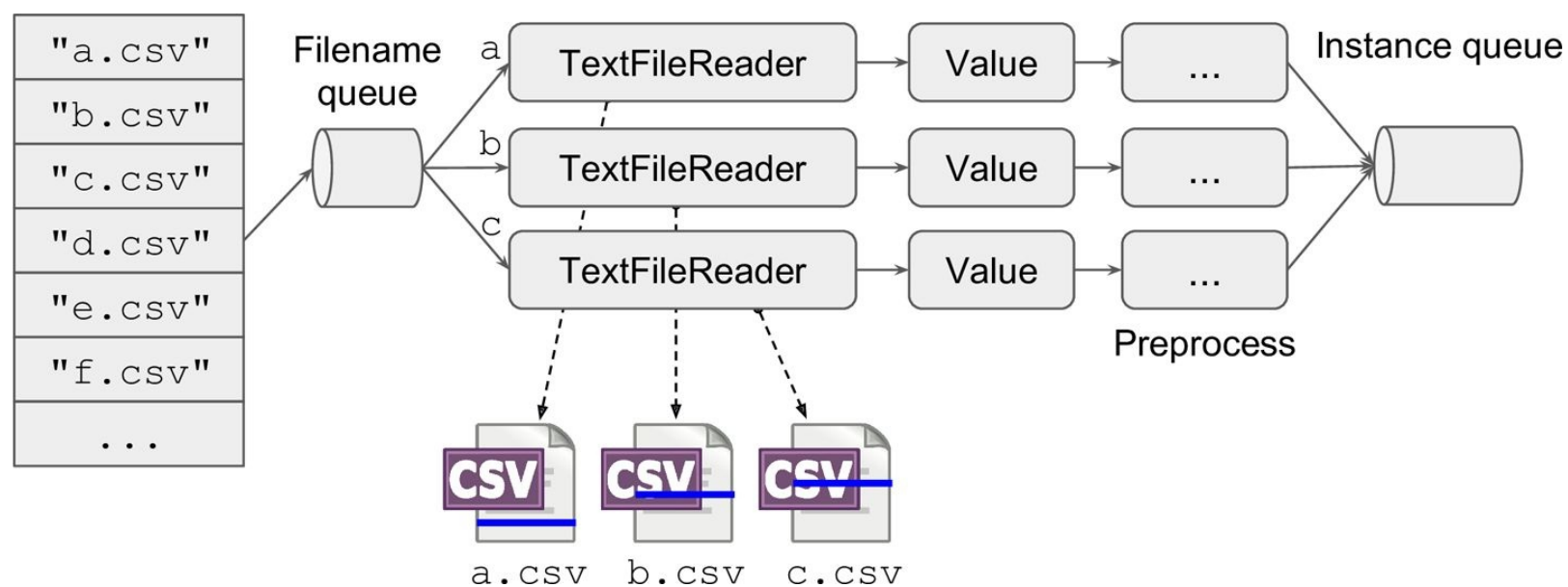
Figure 12-10. Reading simultaneously from multiple files
