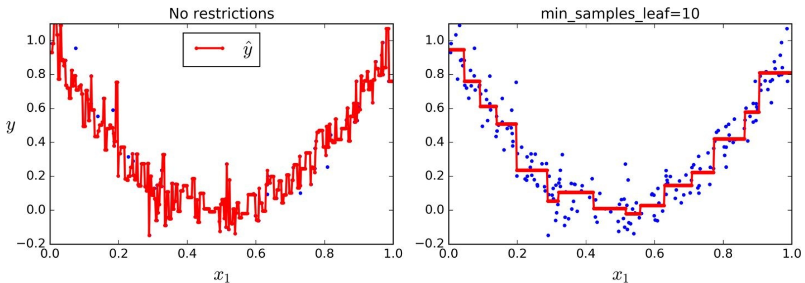
Figure 6-6. Regularizing a Decision Tree regressor
