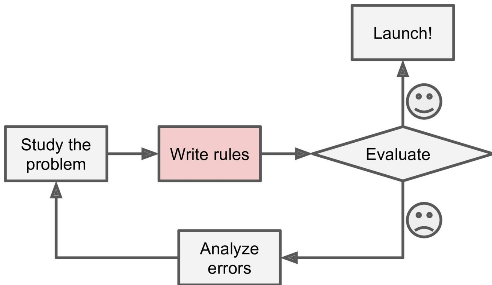
Figure 1-1. The traditional approach
