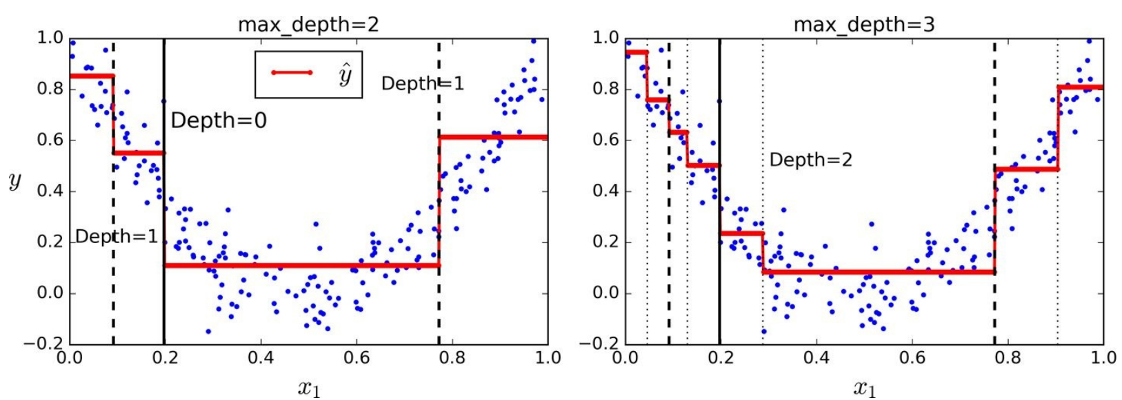
Figure 6-5. Predictions of two Decision Tree regression models
