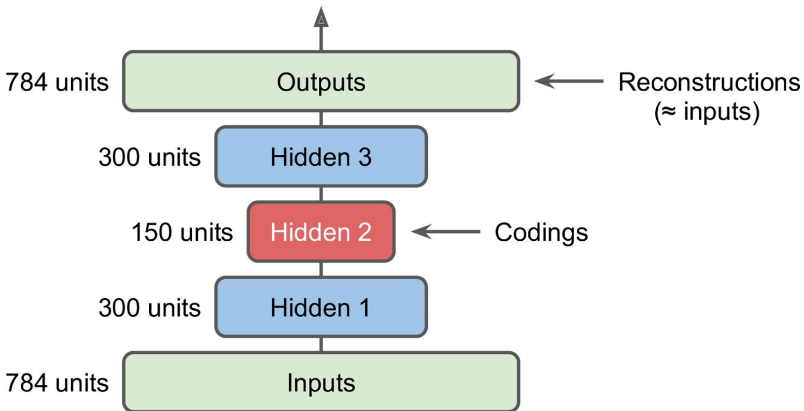
Figure 15-3. Stacked autoencoder
