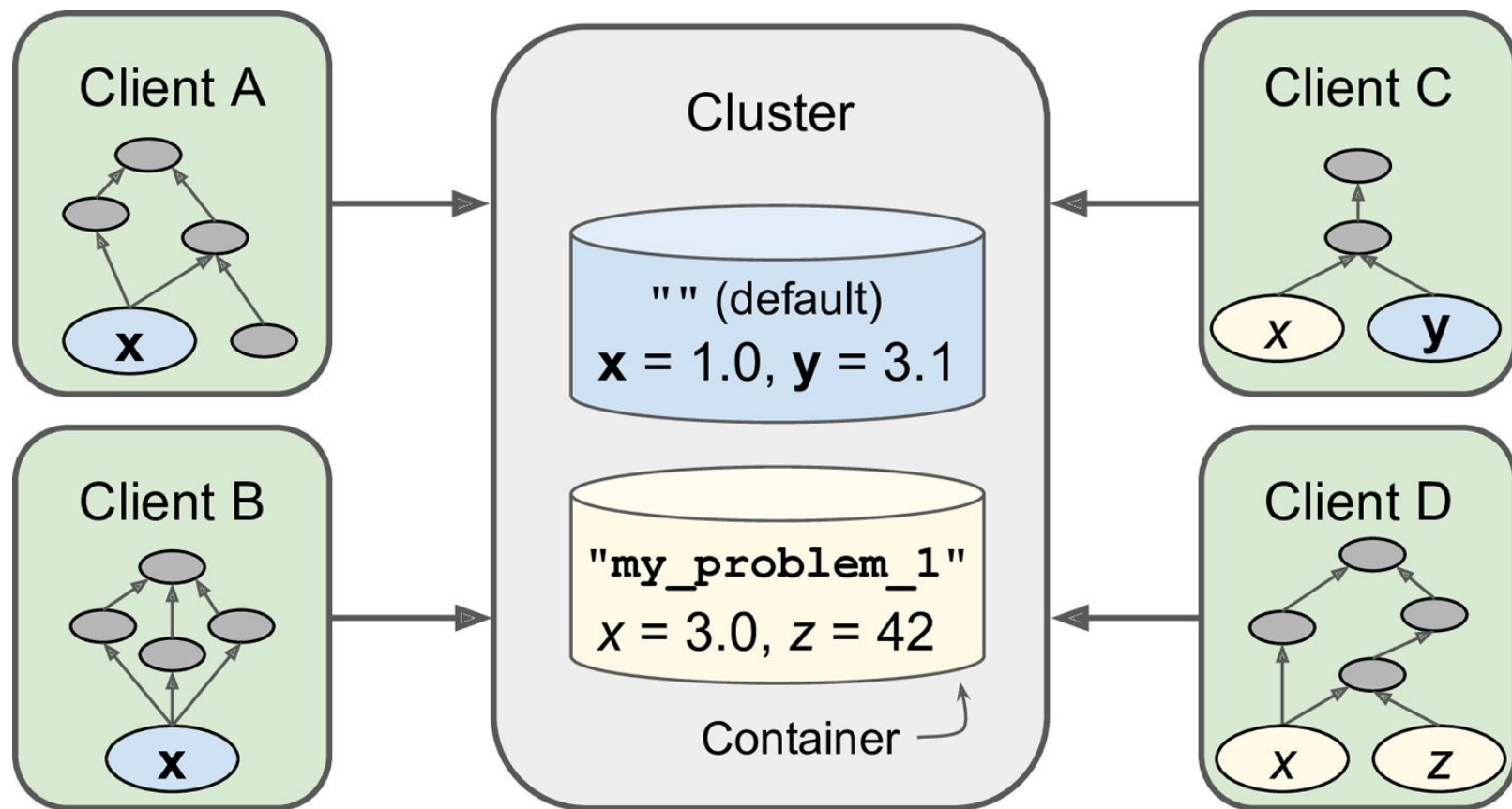
Figure 12-7. Resource containers
