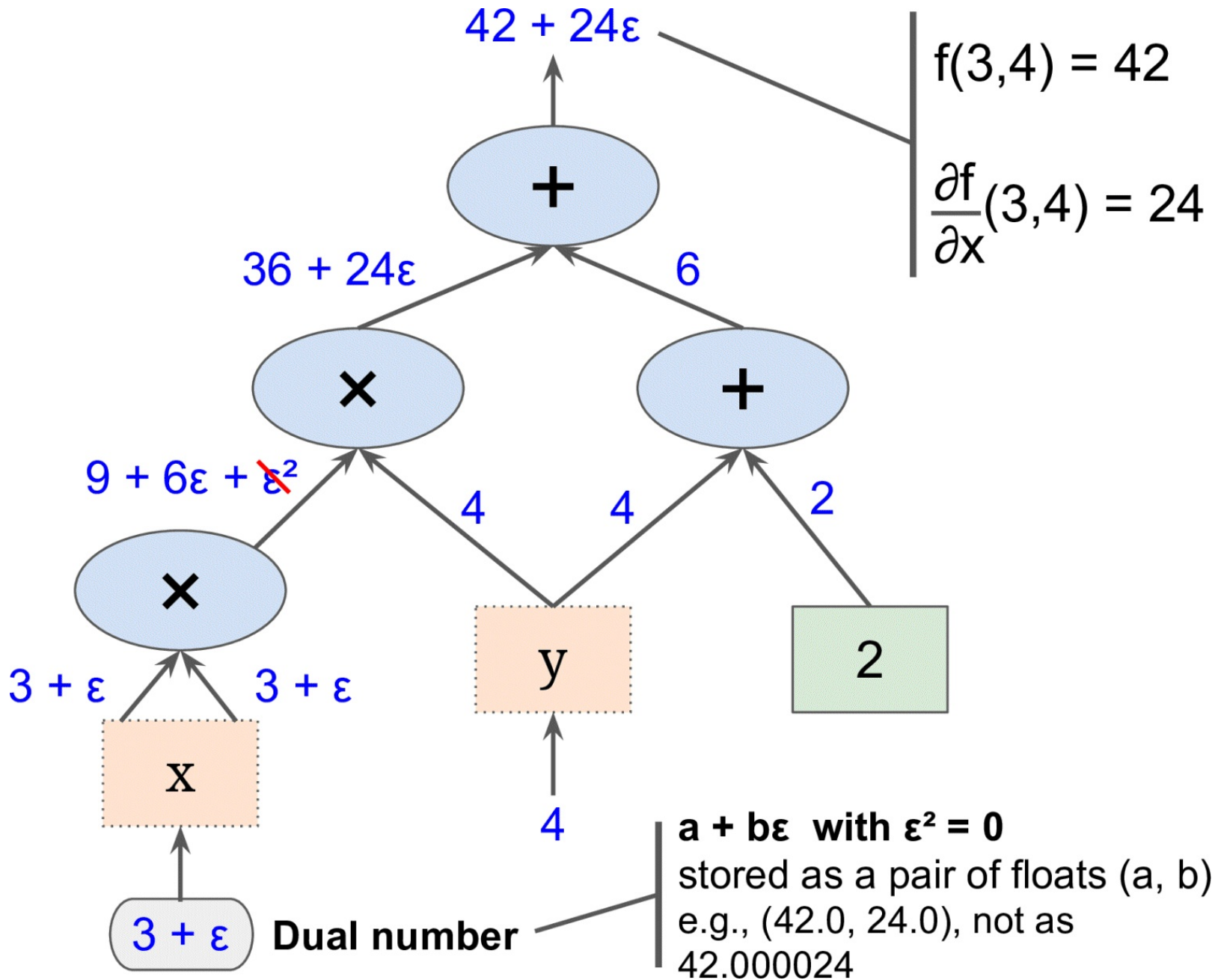
Figure D-2. Forward-mode autodiff
