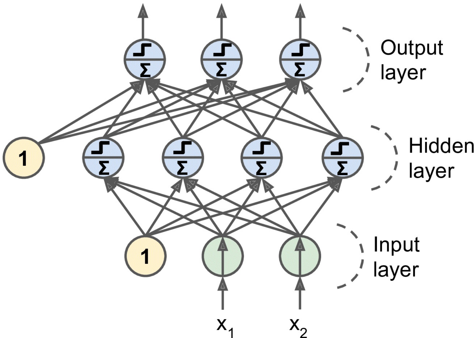
Figure 10-7. Multi-Layer Perceptron
