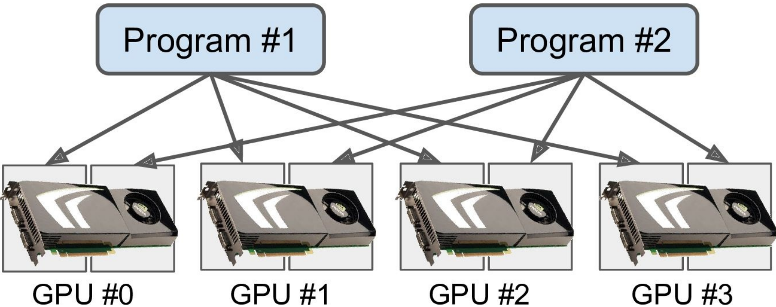
Figure 12-4. Each program gets all four GPUs, but with only 40% of the RAM each
