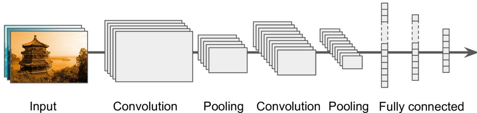
Figure 13-9. Typical CNN architecture
