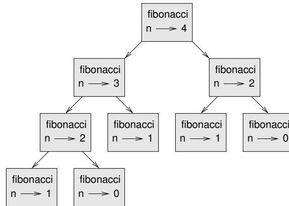
Figure 11.2: Call graph.
