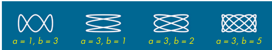
Figure 9-24: Drawing Lissajous curves using different a , b arguments
