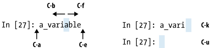
Figure 2-5. Illustration of some keyboard shortcuts in the IPython shell
