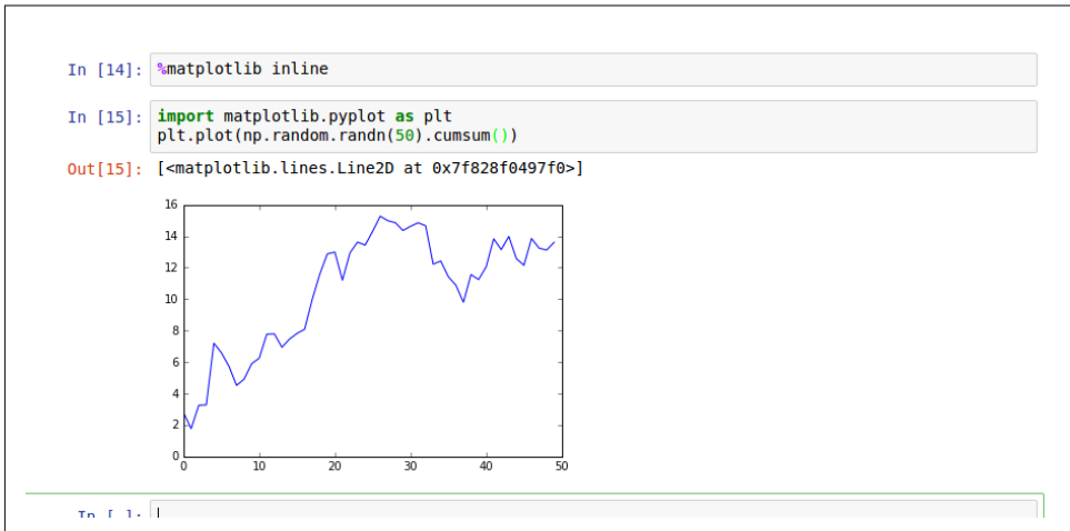
Figure 2-6. Jupyter inline matplotlib plotting
