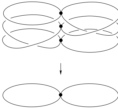
Fig. 12.9: The covering map of Problem 12-3.
