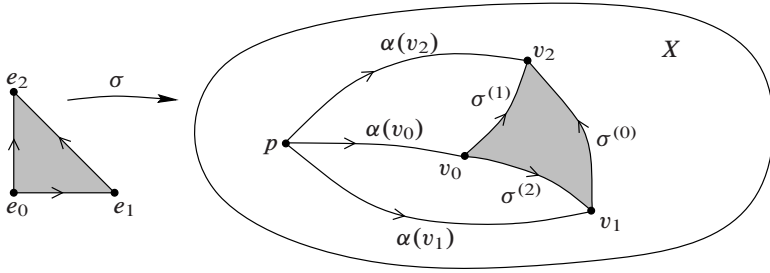
Fig. 13.8: Proof that Ker \gamma is the commutator subgroup.
