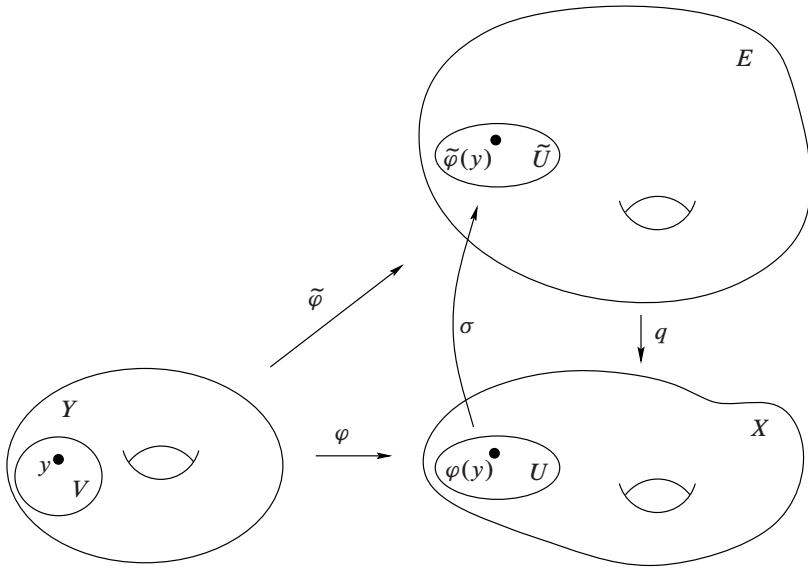
Fig. 11.6: Proof that \tilde{\phi} is continuous.
