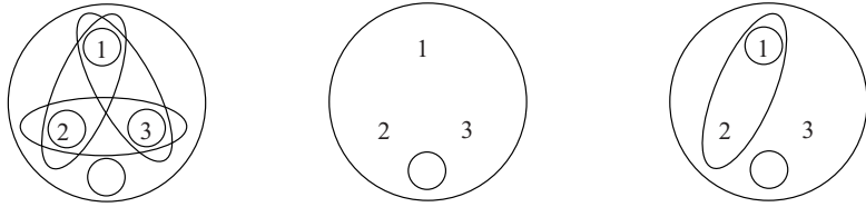
(a) Discrete topology
