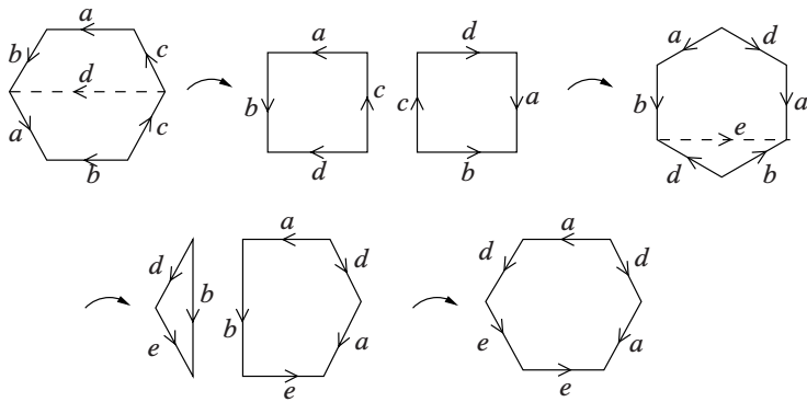
Fig. 6.19: Transforming \mathbb{P}^2 \# \mathbb{P}^2 \# \mathbb{P}^2 to \mathbb{T}^2 \# \mathbb{P}^2 .
