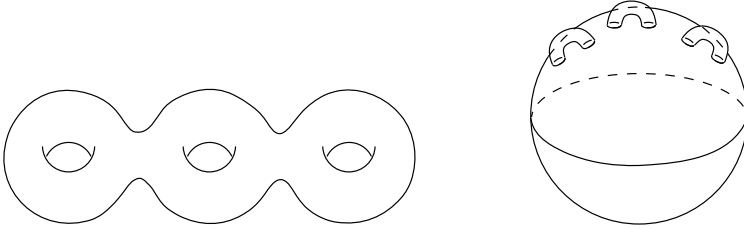
Fig. 6.8: A connected sum of tori.
