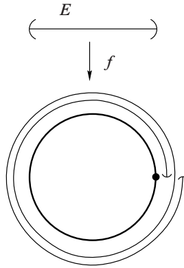
Fig. 11.3: A surjective local homeomorphism that is not a covering map.
