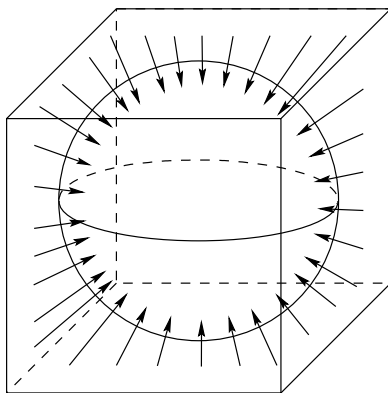
Fig. 2.4: Deforming a cube into a sphere.
