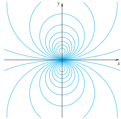
(a) level curves: -3y = c(x^2 + y^2 + 1)
