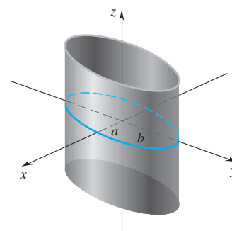
elliptic cylinder
