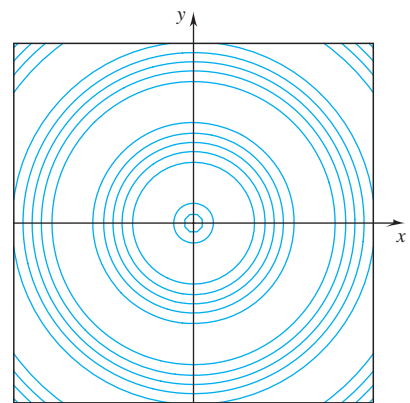
(c) level curves: \sin \sqrt{x^2 + y^2} = c
