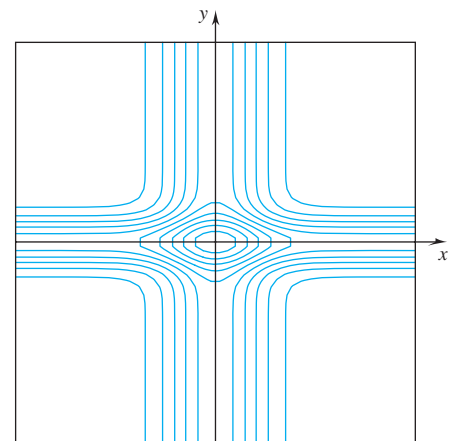
(b) level curves: e^{-x^2} + e^{-4y^2} = c
