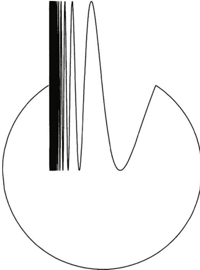
Figure 58 The topologist's sine circle
