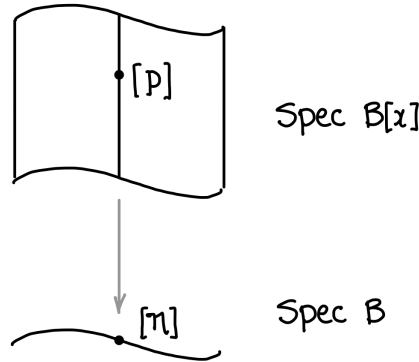
FIGURE 13.4. The geometry behind the proof of Proposition 13.3.7
