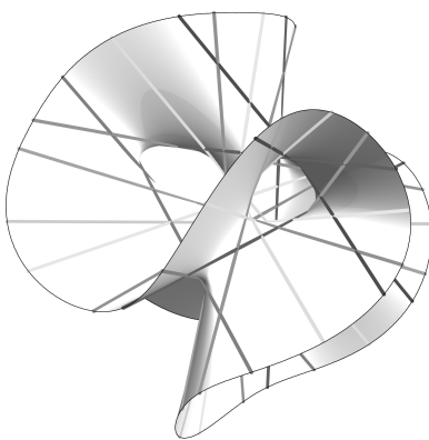
FIGURE 27.1. The twenty-seven lines on the Clebsch cubic surface (from Greg Egan)
