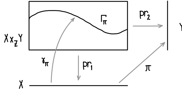
FIGURE 11.2. The graph morphism
