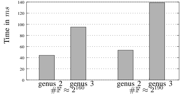
Fig. 1. Timings of Scalar Multiplication for Different Group Orders and Genera (ARM7TDMI@80MHz)
