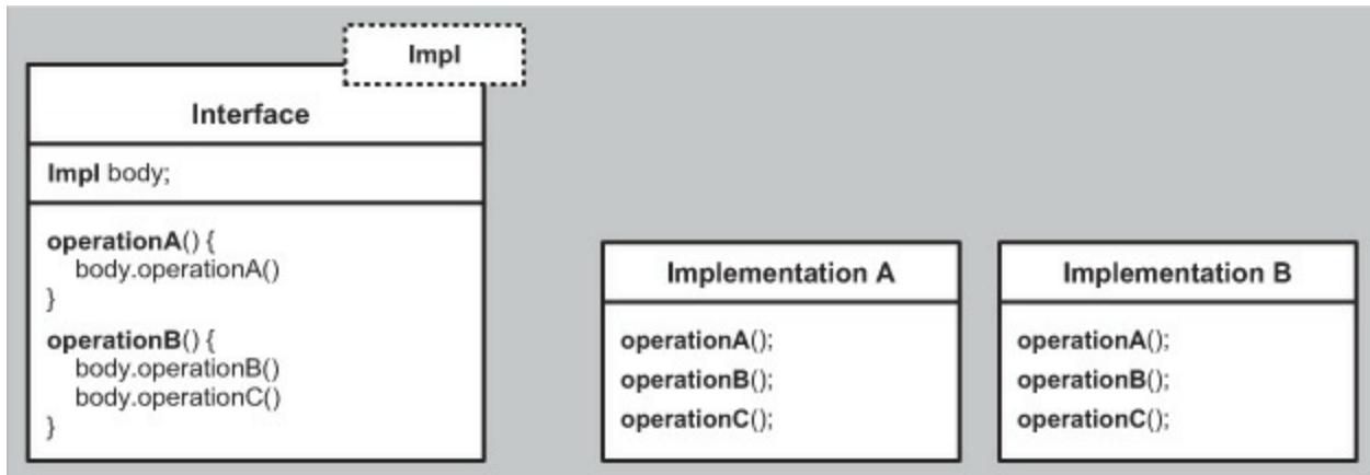
Figure 18.4. Bridge pattern implemented using templates
