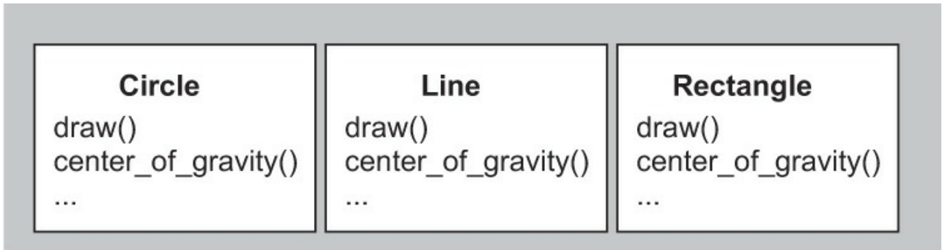
Figure 18.2. Polymorphism implemented via templates
