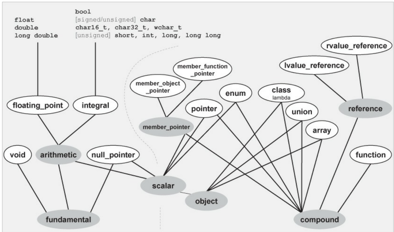
Figure D.1. Primary and Composite Type Categories
