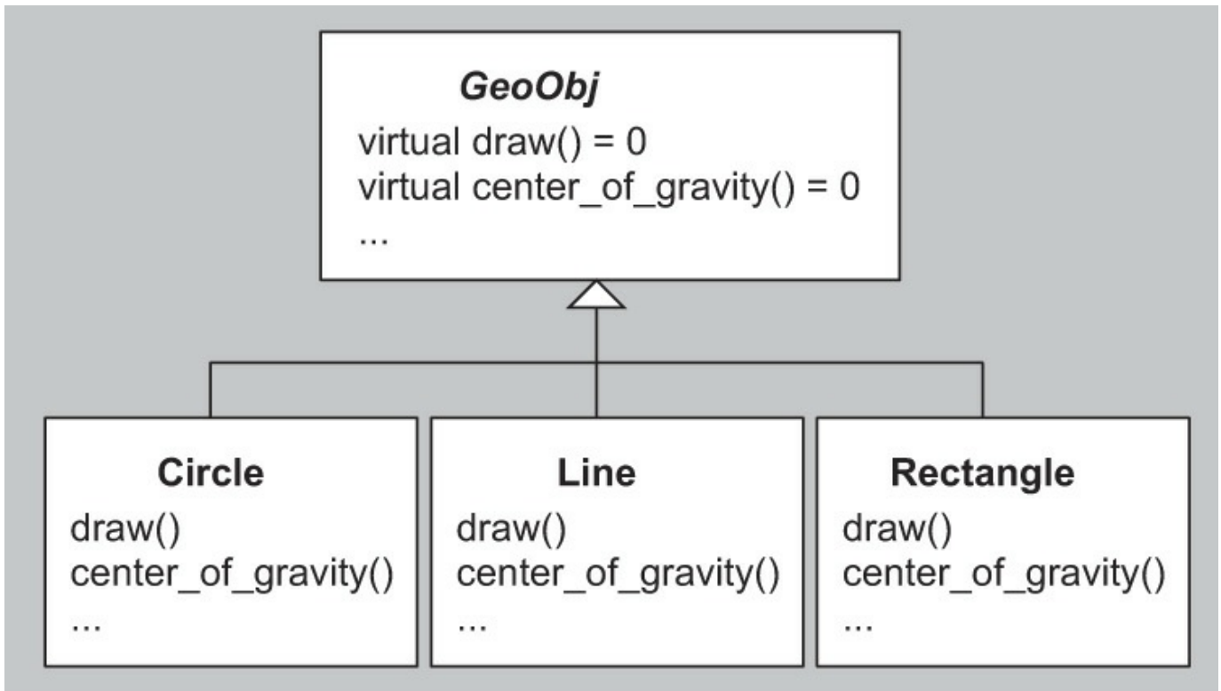
Figure 18.1. Polymorphism implemented via inheritance
