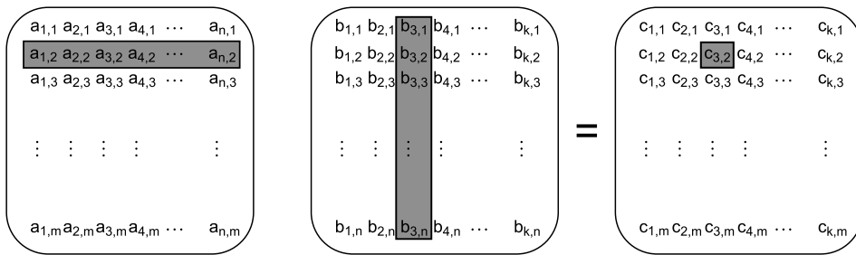
Figure 8.3 Matrix multiplication
